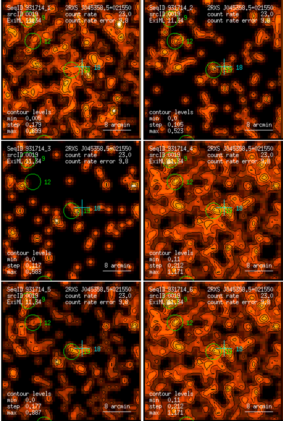
Figure 19: RASS 931714: detection 0019: band rate images, Gaussian filter: (1) PSPC channels 11 – 41, (2) 52 – 90, (3) 91 – 201, (4) 11 – 235, (5) 52 – 201, (6) 11 – 201. Broad band rates in counts/ks. Band rate contour levels in counts/ks/arcmin 2 .
