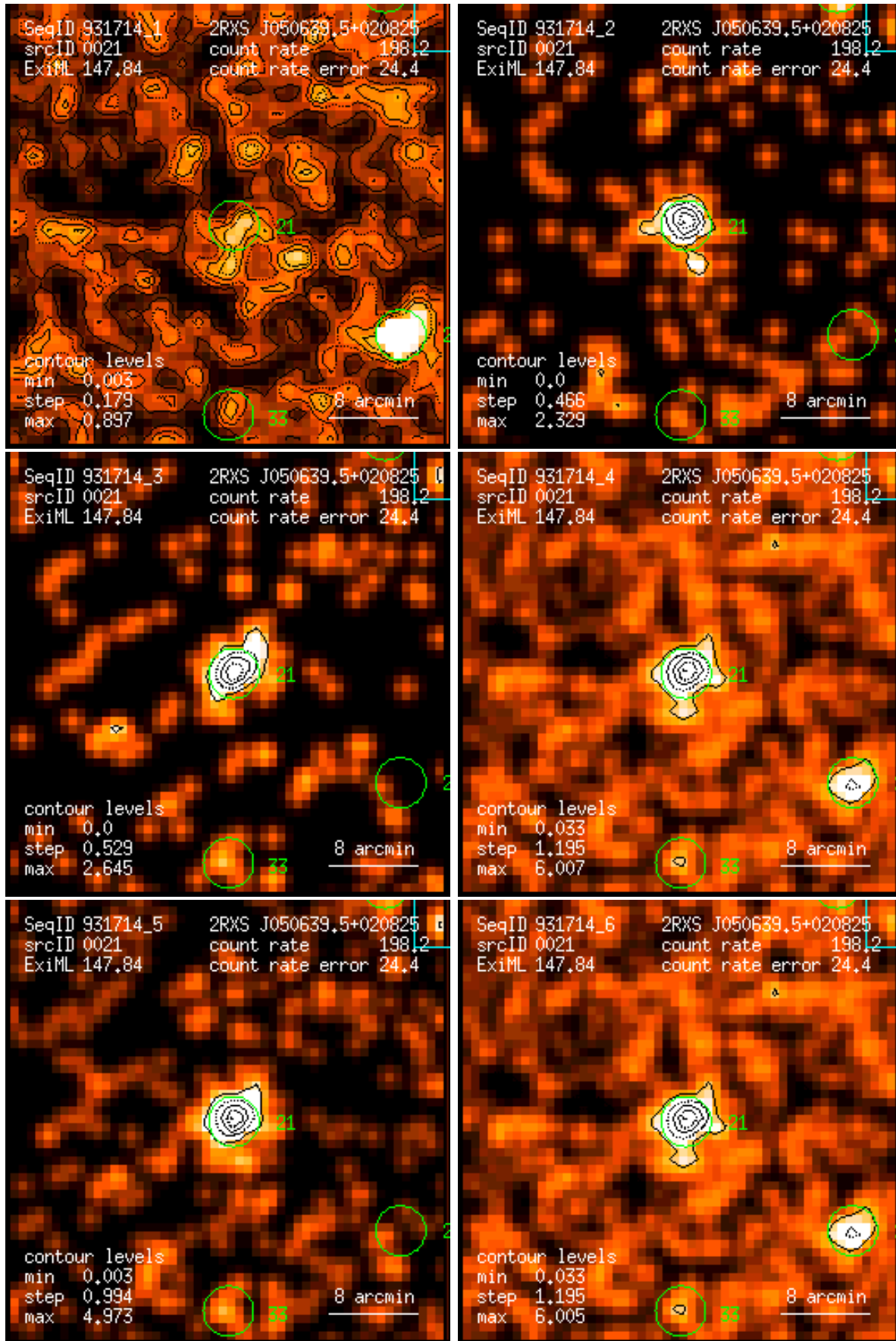
Figure 21: RASS 931714: detection 0021: band rate images, Gaussian filter: (1) PSPC channels 11 – 41, (2) 52 – 90, (3) 91 – 201, (4) 11 – 235, (5) 52 – 201, (6) 11 – 201. Broad band rates in counts/ks. Band rate contour levels in counts/ks/arcmin 2 .
