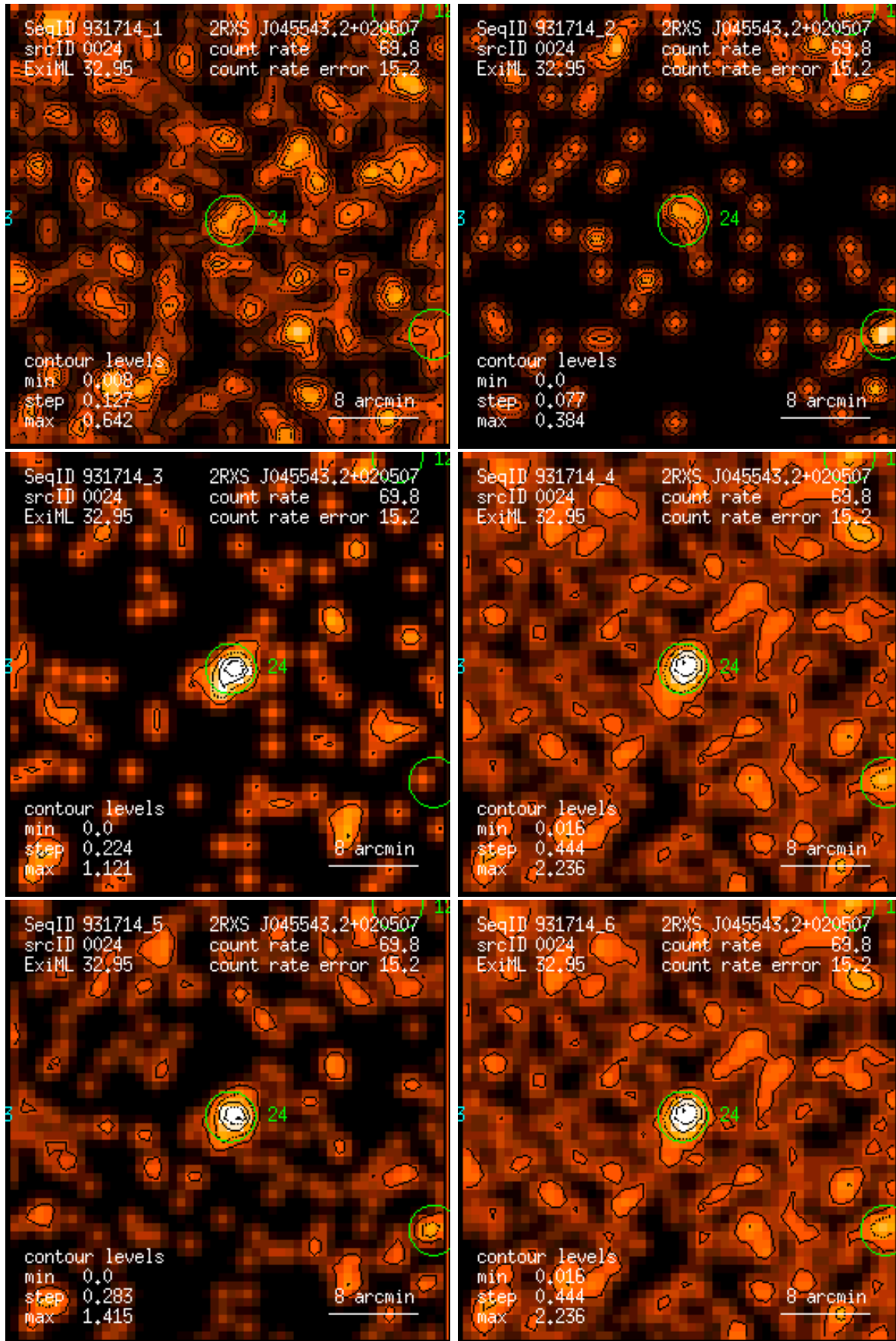
Figure 24: RASS 931714: detection 0024: band rate images, Gaussian filter: (1) PSPC channels 11 – 41, (2) 52 – 90, (3) 91 – 201, (4) 11 – 235, (5) 52 – 201, (6) 11 – 201. Broad band rates in counts/ks. Band rate contour levels in counts/ks/arcmin 2 .
