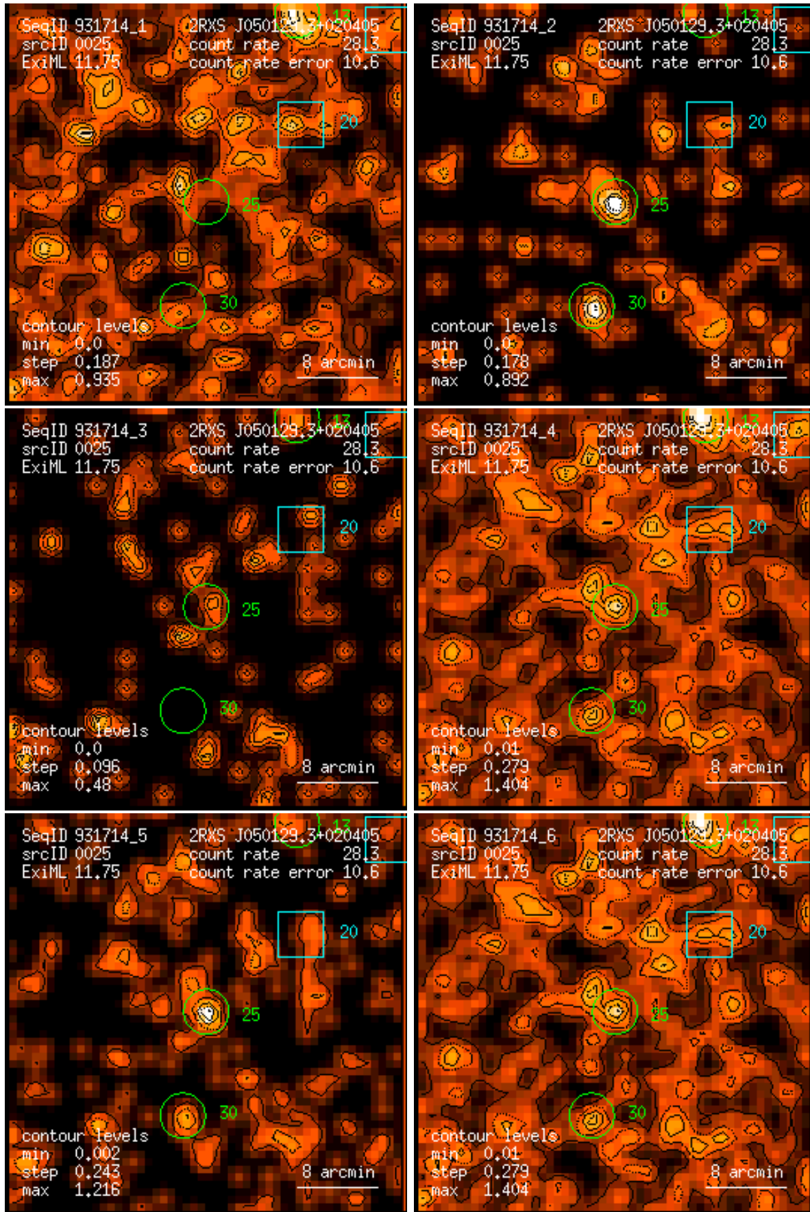
Figure 25: RASS 931714: detection 0025: band rate images, Gaussian filter: (1) PSPC channels 11 – 41, (2) 52 – 90, (3) 91 – 201, (4) 11 – 235, (5) 52 – 201, (6) 11 – 201. Broad band rates in counts/ks. Band rate contour levels in counts/ks/arcmin 2 .
