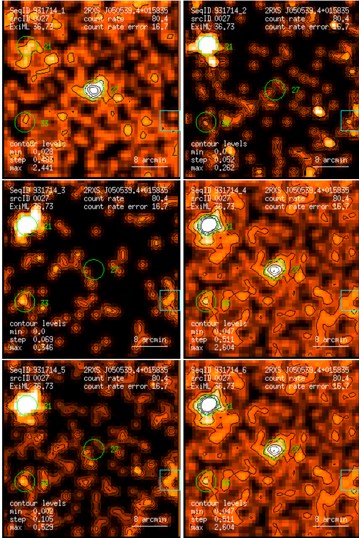
Figure 27: RASS 931714: detection 0027: band rate images, Gaussian filter: (1) PSPC channels 11 – 41, (2) 52 – 90, (3) 91 – 201, (4) 11 – 235, (5) 52 – 201, (6) 11 – 201. Broad band rates in counts/ks. Band rate contour levels in counts/ks/arcmin 2 .
