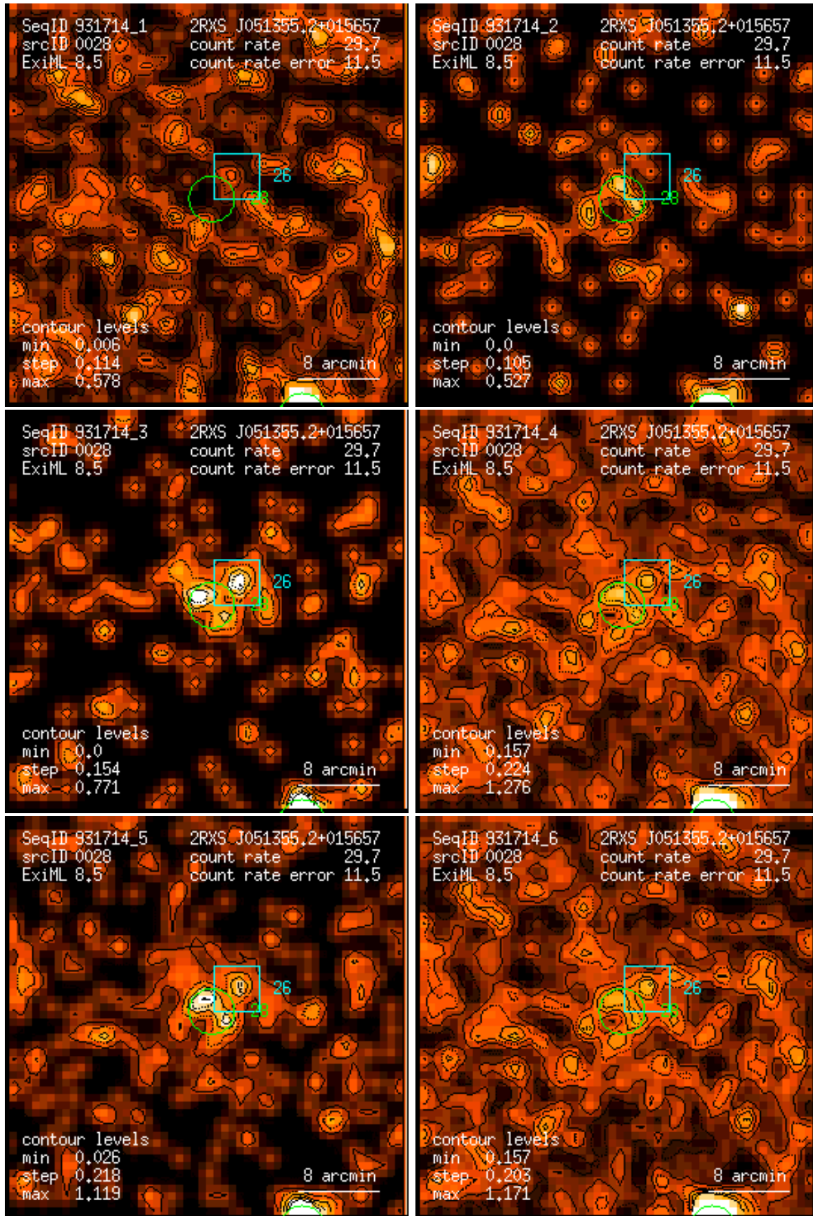
Figure 28: RASS 931714: detection 0028: band rate images, Gaussian filter: (1) PSPC channels 11 – 41, (2) 52 – 90, (3) 91 – 201, (4) 11 – 235, (5) 52 – 201, (6) 11 – 201. Broad band rates in counts/ks. Band rate contour levels in counts/ks/arcmin 2 .
