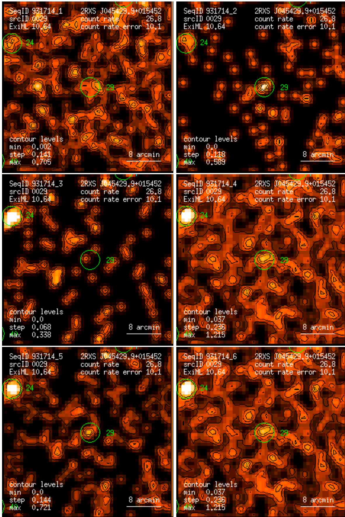
Figure 29: RASS 931714: detection 0029: band rate images, Gaussian filter: (1) PSPC channels 11 – 41, (2) 52 – 90, (3) 91 – 201, (4) 11 – 235, (5) 52 – 201, (6) 11 – 201. Broad band rates in counts/ks. Band rate contour levels in counts/ks/arcmin 2 .
