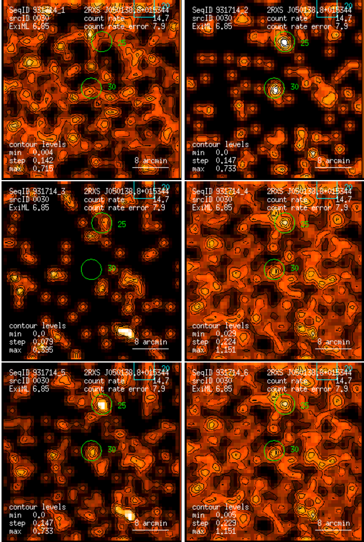
Figure 30: RASS 931714: detection 0030: band rate images, Gaussian filter: (1) PSPC channels 11 – 41, (2) 52 – 90, (3) 91 – 201, (4) 11 – 235, (5) 52 – 201, (6) 11 – 201. Broad band rates in counts/ks. Band rate contour levels in counts/ks/arcmin 2 .
