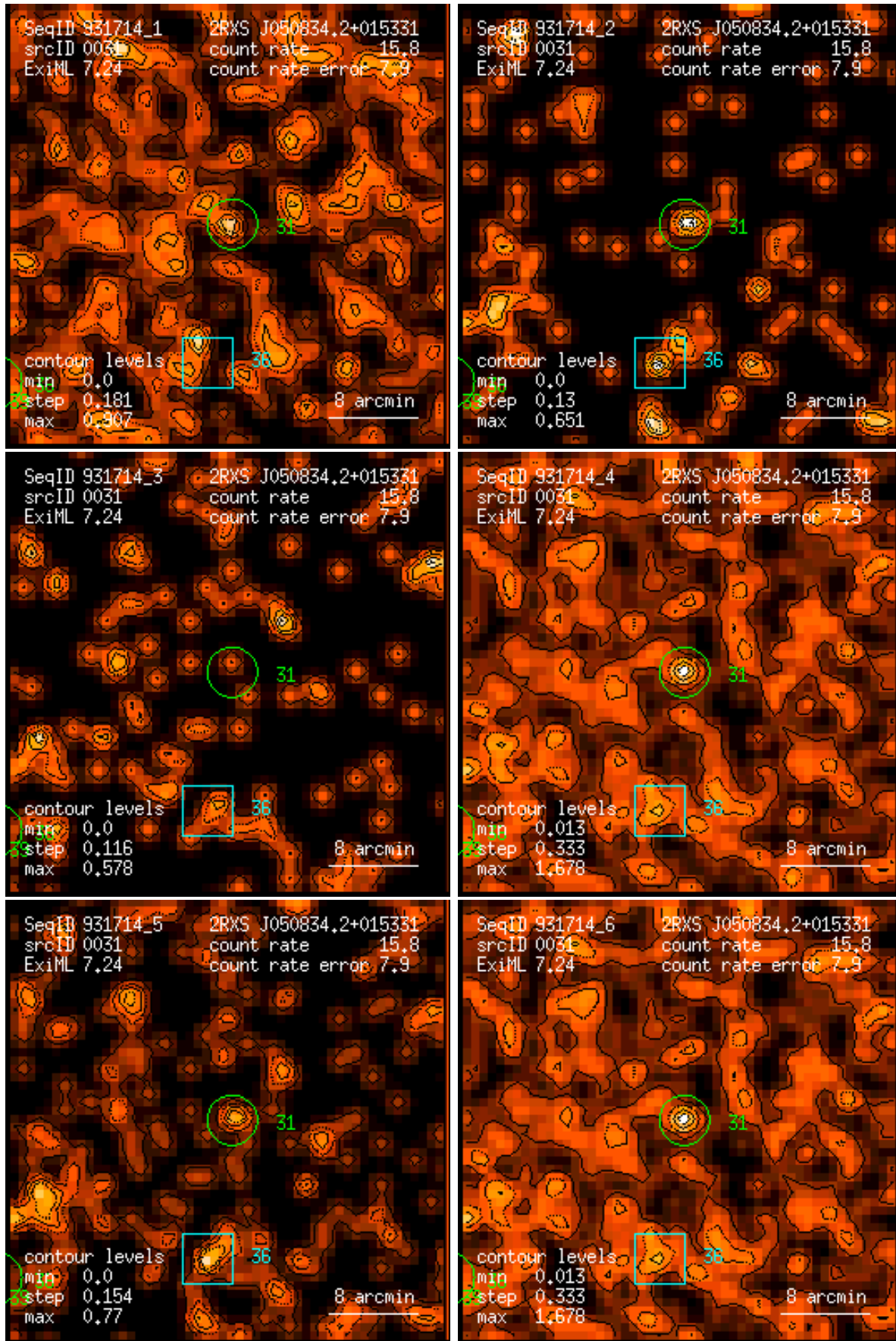
Figure 31: RASS 931714: detection 0031: band rate images, Gaussian filter: (1) PSPC channels 11 – 41, (2) 52 – 90, (3) 91 – 201, (4) 11 – 235, (5) 52 – 201, (6) 11 – 201. Broad band rates in counts/ks. Band rate contour levels in counts/ks/arcmin 2 .
