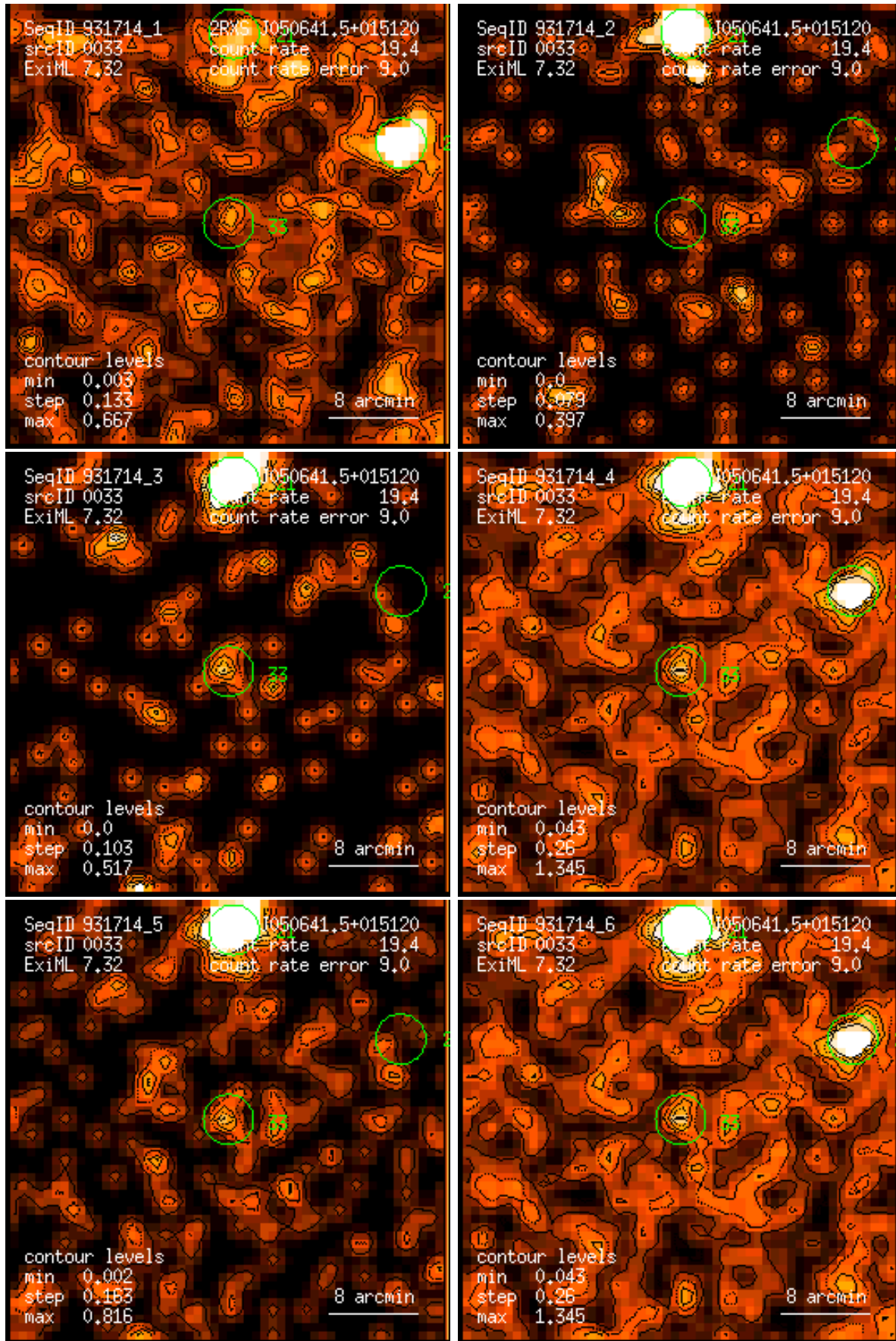
Figure 33: RASS 931714: detection 0033: band rate images, Gaussian filter: (1) PSPC channels 11 – 41, (2) 52 – 90, (3) 91 – 201, (4) 11 – 235, (5) 52 – 201, (6) 11 – 201. Broad band rates in counts/ks. Band rate contour levels in counts/ks/arcmin 2 .
