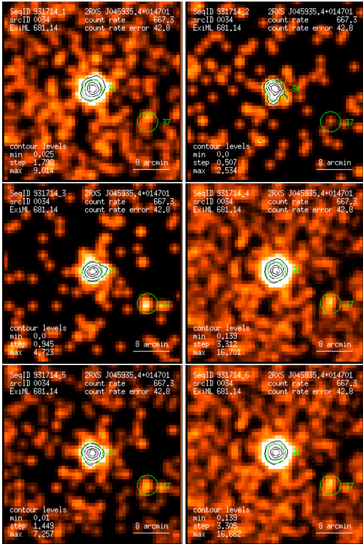
Figure 34: RASS 931714: detection 0034: band rate images, Gaussian filter: (1) PSPC channels 11 – 41, (2) 52 – 90, (3) 91 – 201, (4) 11 – 235, (5) 52 – 201, (6) 11 – 201. Broad band rates in counts/ks. Band rate contour levels in counts/ks/arcmin 2 .
