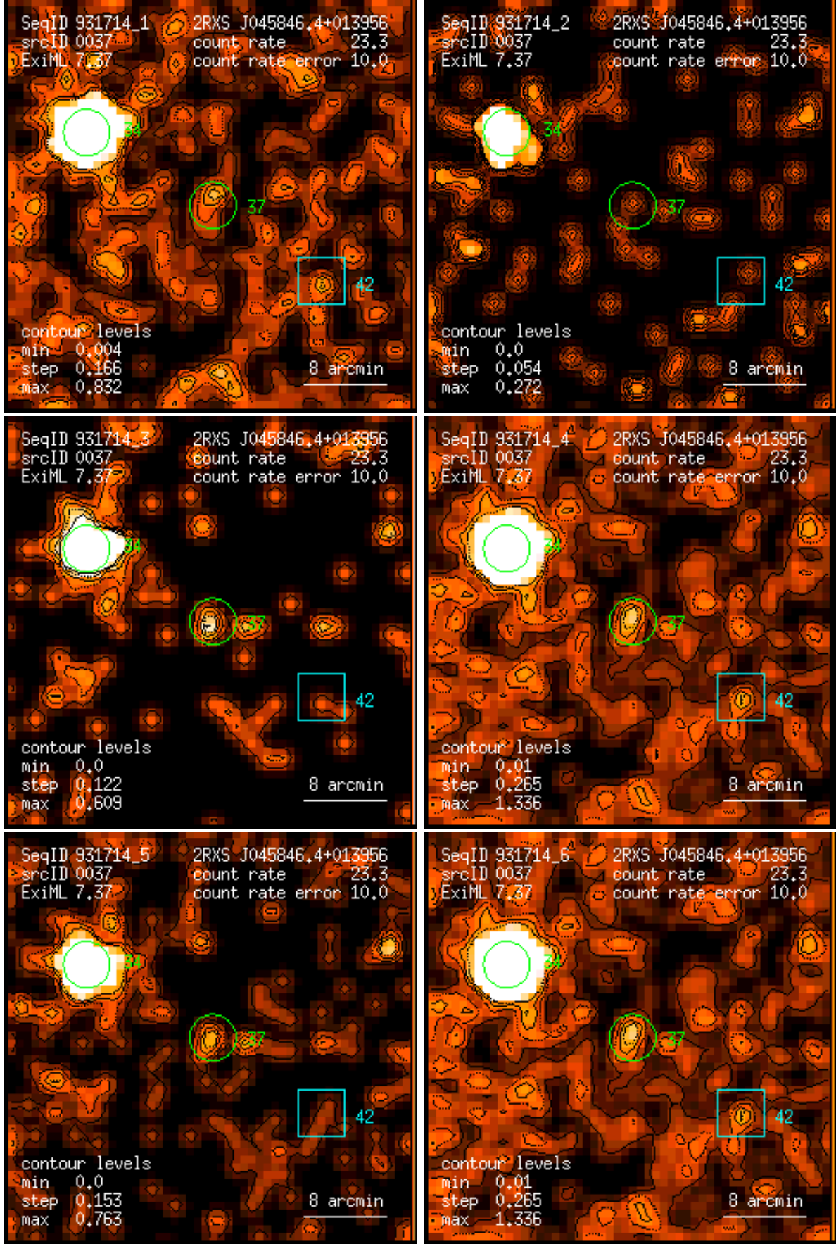
Figure 37: RASS 931714: detection 0037: band rate images, Gaussian filter: (1) PSPC channels 11 – 41, (2) 52 – 90, (3) 91 – 201, (4) 11 – 235, (5) 52 – 201, (6) 11 – 201. Broad band rates in counts/ks. Band rate contour levels in counts/ks/arcmin 2 .
