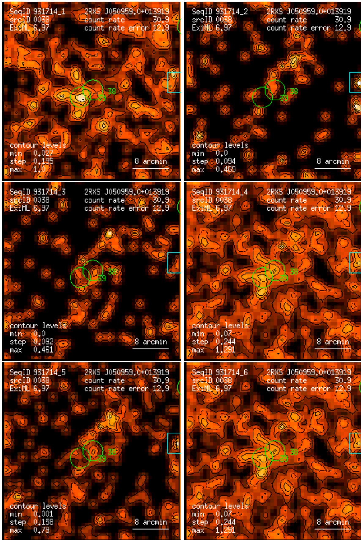
Figure 38: RASS 931714: detection 0038: band rate images, Gaussian filter: (1) PSPC channels 11 – 41, (2) 52 – 90, (3) 91 – 201, (4) 11 – 235, (5) 52 – 201, (6) 11 – 201. Broad band rates in counts/ks. Band rate contour levels in counts/ks/arcmin 2 .
