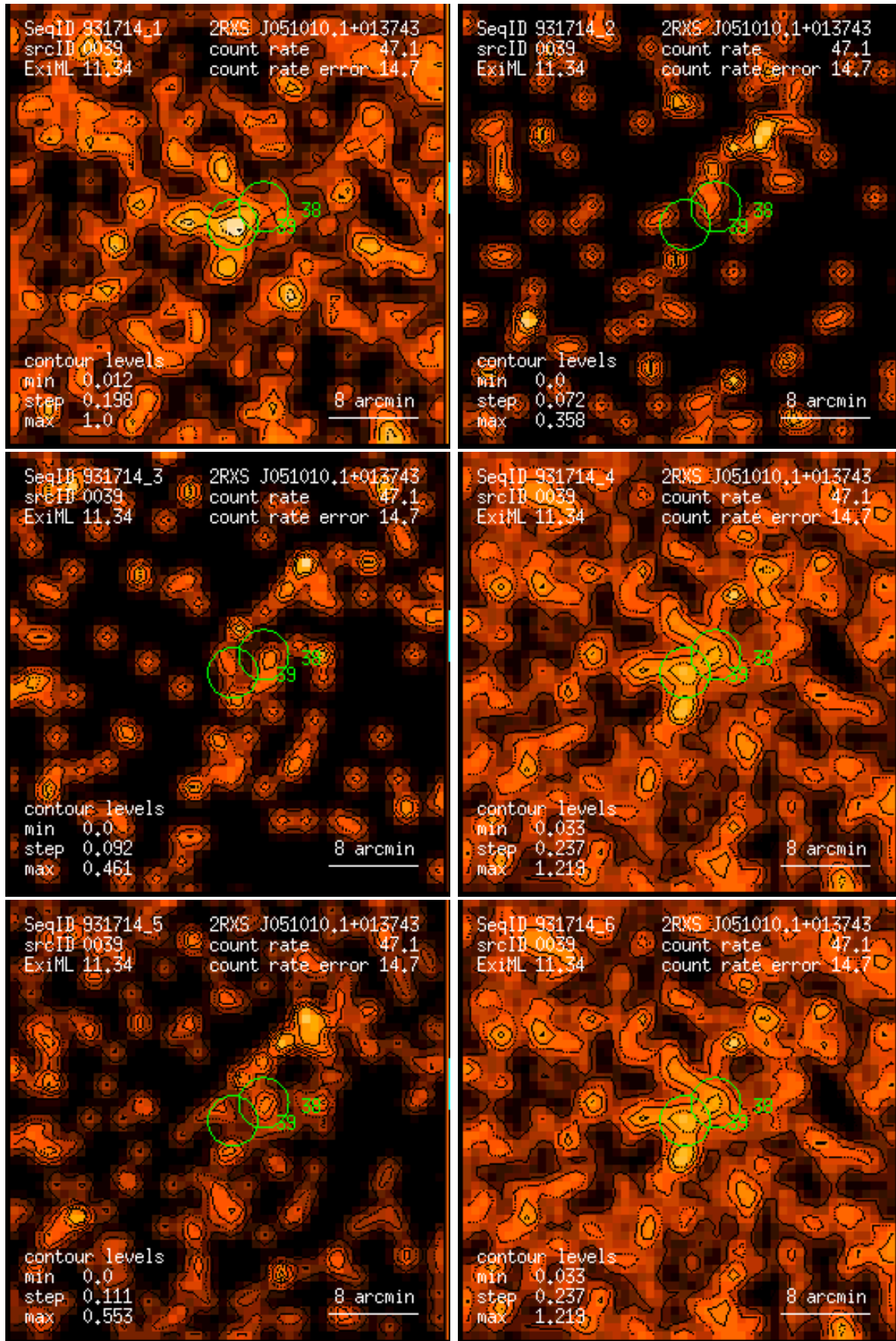
Figure 39: RASS 931714: detection 0039: band rate images, Gaussian filter: (1) PSPC channels 11 – 41, (2) 52 – 90, (3) 91 – 201, (4) 11 – 235, (5) 52 – 201, (6) 11 – 201. Broad band rates in counts/ks. Band rate contour levels in counts/ks/arcmin 2 .
