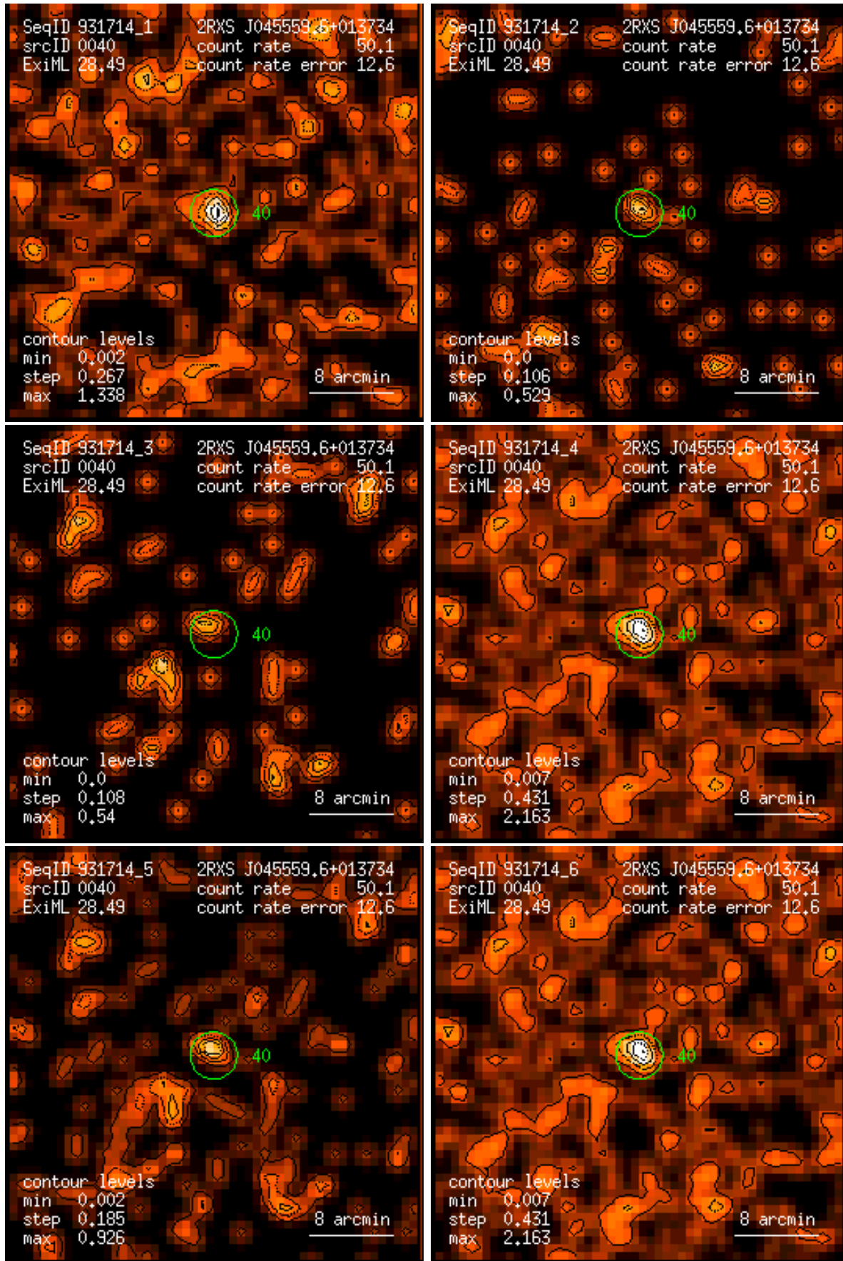
Figure 40: RASS 931714: detection 0040: band rate images, Gaussian filter: (1) PSPC channels 11 – 41, (2) 52 – 90, (3) 91 – 201, (4) 11 – 235, (5) 52 – 201, (6) 11 – 201. Broad band rates in counts/ks. Band rate contour levels in counts/ks/arcmin 2 .
