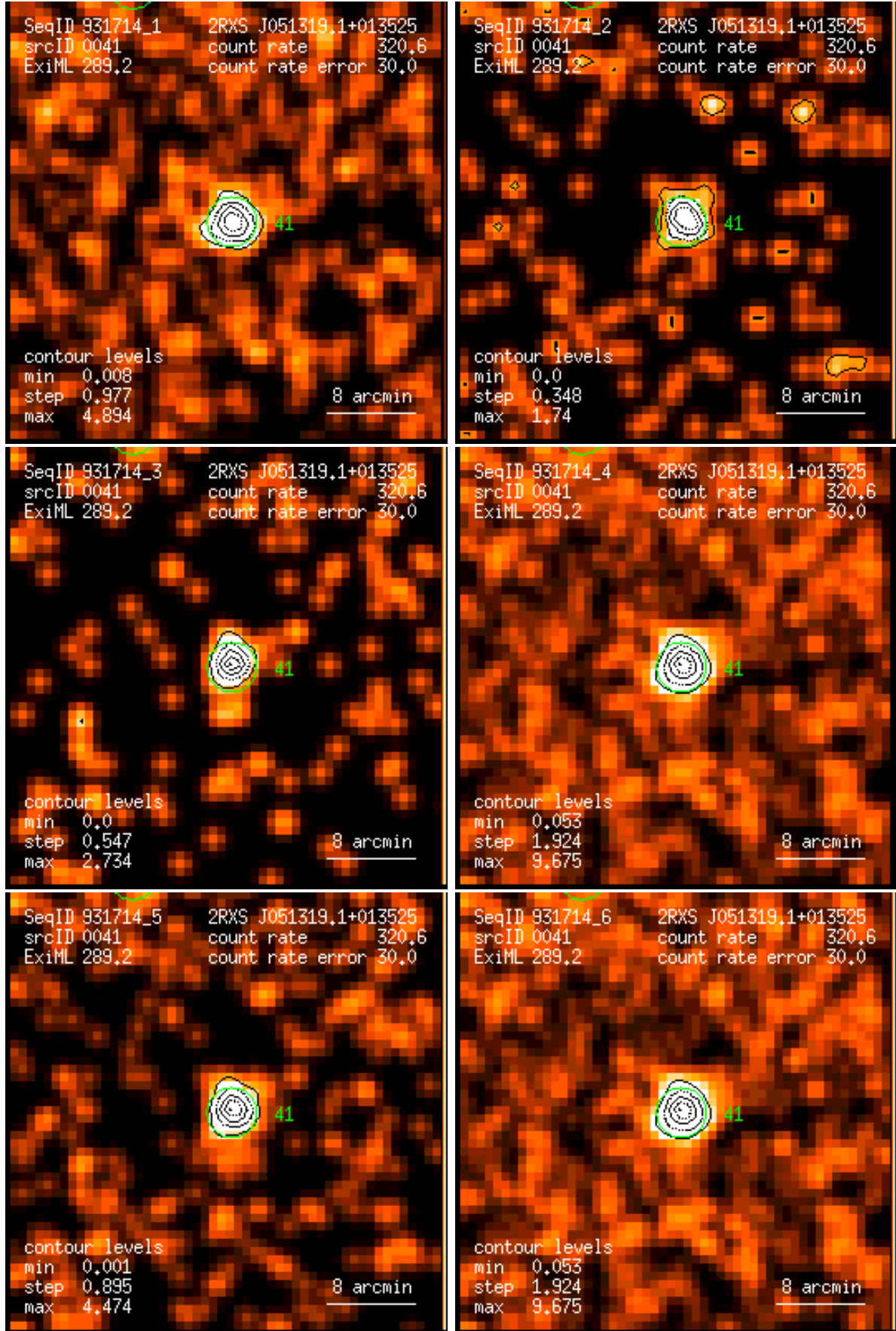
Figure 41: RASS 931714: detection 0041: band rate images, Gaussian filter: (1) PSPC channels 11 – 41, (2) 52 – 90, (3) 91 – 201, (4) 11 – 235, (5) 52 – 201, (6) 11 – 201. Broad band rates in counts/ks. Band rate contour levels in counts/ks/arcmin 2 .
