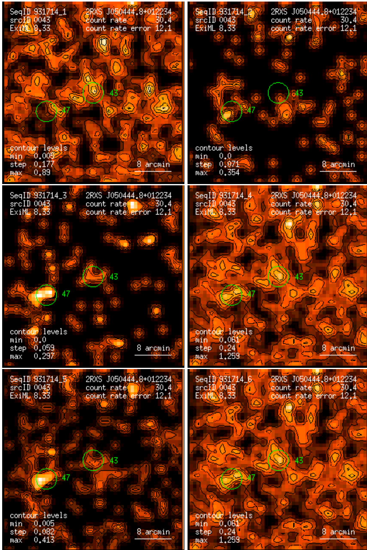
Figure 43: RASS 931714: detection 0043: band rate images, Gaussian filter: (1) PSPC channels 11 – 41, (2) 52 – 90, (3) 91 – 201, (4) 11 – 235, (5) 52 – 201, (6) 11 – 201. Broad band rates in counts/ks. Band rate contour levels in counts/ks/arcmin 2 .
