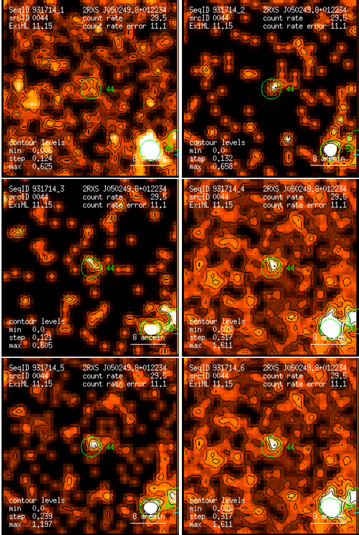
Figure 44: RASS 931714: detection 0044: band rate images, Gaussian filter: (1) PSPC channels 11 – 41, (2) 52 – 90, (3) 91 – 201, (4) 11 – 235, (5) 52 – 201, (6) 11 – 201. Broad band rates in counts/ks. Band rate contour levels in counts/ks/arcmin 2 .
