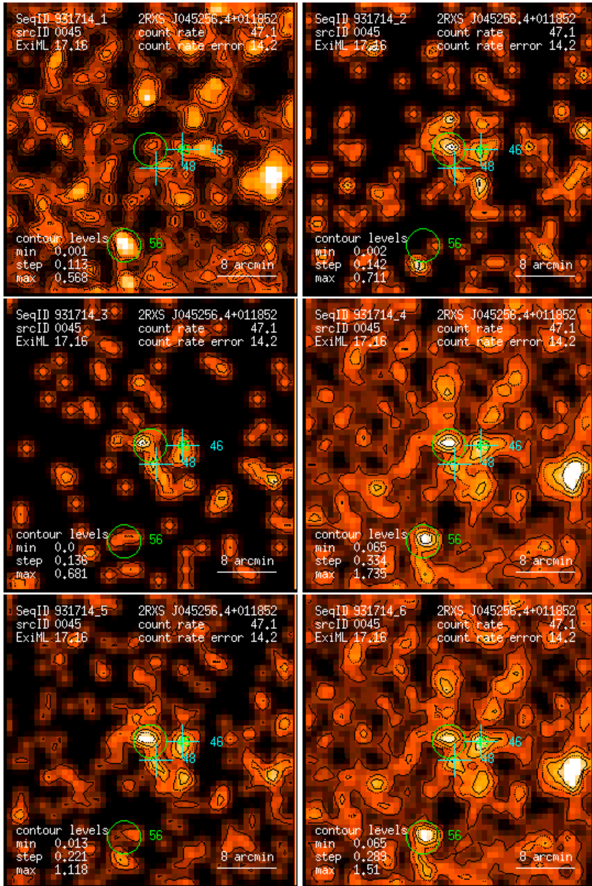
Figure 45: RASS 931714: detection 0045: band rate images, Gaussian filter: (1) PSPC channels 11 – 41, (2) 52 – 90, (3) 91 – 201, (4) 11 – 235, (5) 52 – 201, (6) 11 – 201. Broad band rates in counts/ks. Band rate contour levels in counts/ks/arcmin 2 .
