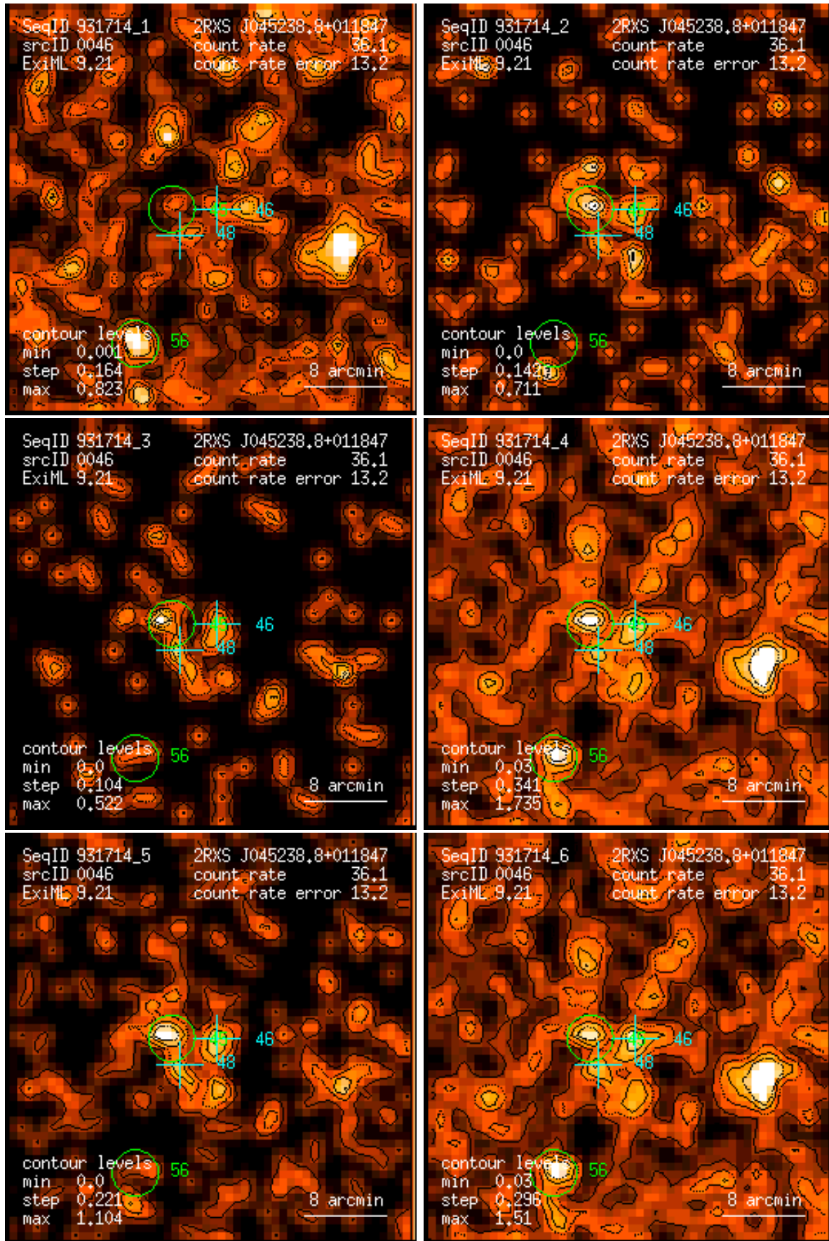
Figure 46: RASS 931714: detection 0046: band rate images, Gaussian filter: (1) PSPC channels 11 – 41, (2) 52 – 90, (3) 91 – 201, (4) 11 – 235, (5) 52 – 201, (6) 11 – 201. Broad band rates in counts/ks. Band rate contour levels in counts/ks/arcmin 2 .
