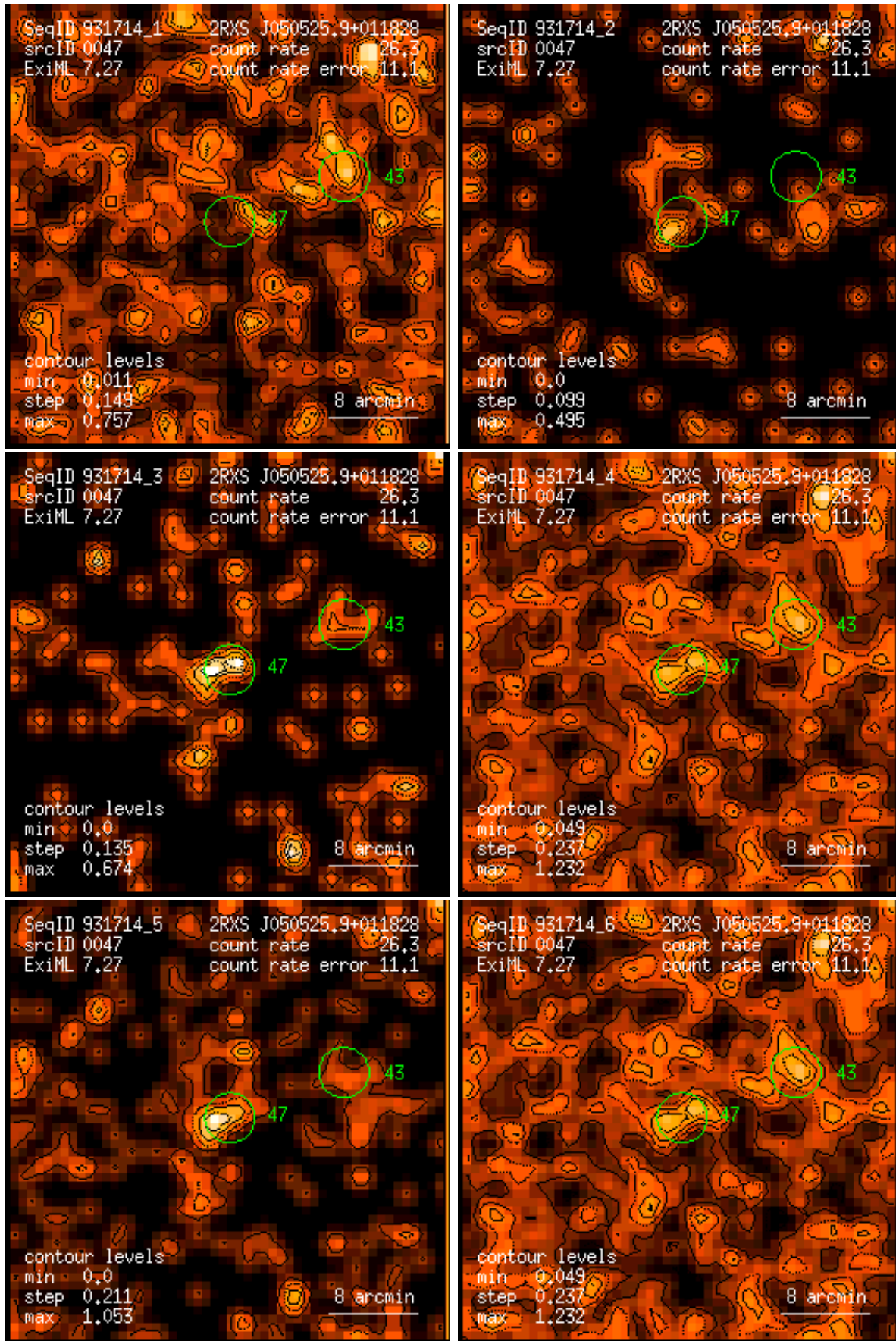
Figure 47: RASS 931714: detection 0047: band rate images, Gaussian filter: (1) PSPC channels 11 – 41, (2) 52 – 90, (3) 91 – 201, (4) 11 – 235, (5) 52 – 201, (6) 11 – 201. Broad band rates in counts/ks. Band rate contour levels in counts/ks/arcmin 2 .
