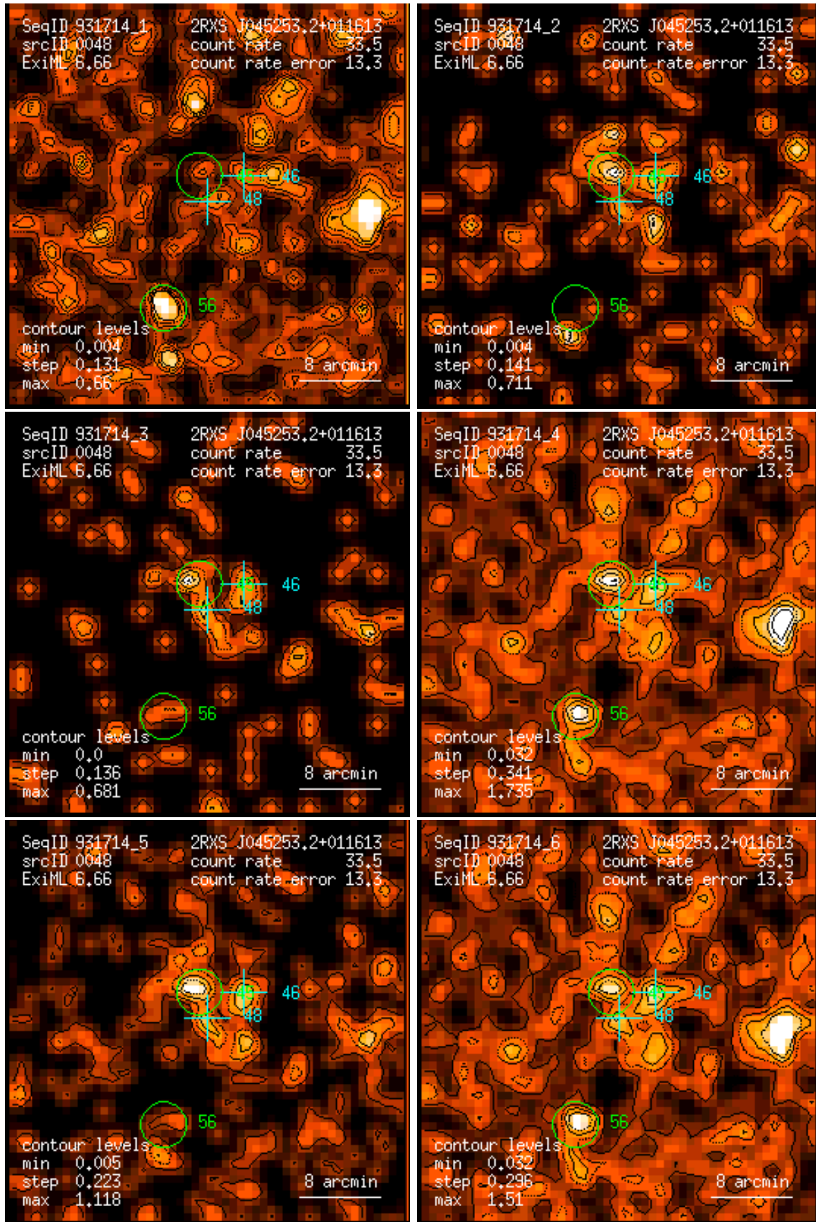
Figure 48: RASS 931714: detection 0048: band rate images, Gaussian filter: (1) PSPC channels 11 – 41, (2) 52 – 90, (3) 91 – 201, (4) 11 – 235, (5) 52 – 201, (6) 11 – 201. Broad band rates in counts/ks. Band rate contour levels in counts/ks/arcmin 2 .
