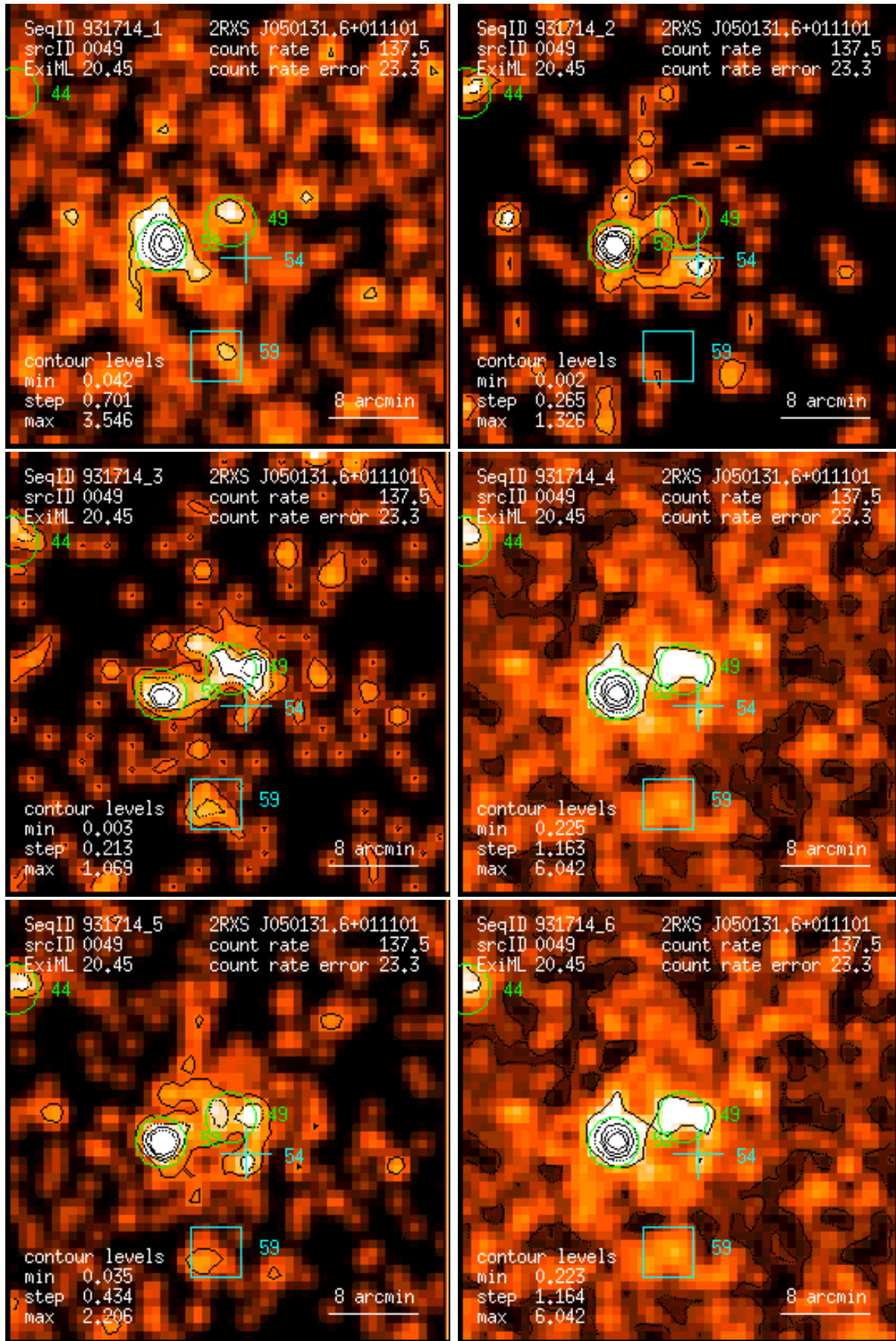
Figure 49: RASS 931714: detection 0049: band rate images, Gaussian filter: (1) PSPC channels 11 – 41, (2) 52 – 90, (3) 91 – 201, (4) 11 – 235, (5) 52 – 201, (6) 11 – 201. Broad band rates in counts/ks. Band rate contour levels in counts/ks/arcmin 2 .
