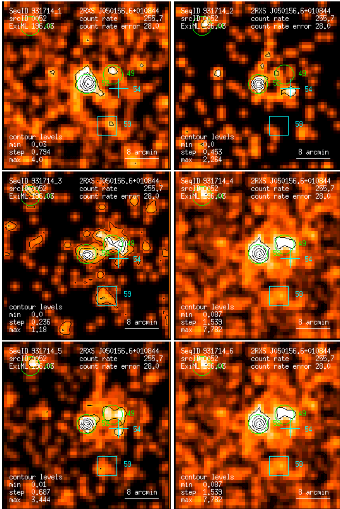
Figure 52: RASS 931714: detection 0052: band rate images, Gaussian filter: (1) PSPC channels 11 – 41, (2) 52 – 90, (3) 91 – 201, (4) 11 – 235, (5) 52 – 201, (6) 11 – 201. Broad band rates in counts/ks. Band rate contour levels in counts/ks/arcmin 2 .
