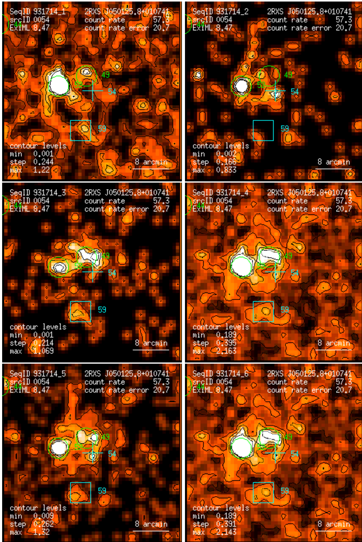
Figure 54: RASS 931714: detection 0054: band rate images, Gaussian filter: (1) PSPC channels 11 – 41, (2) 52 – 90, (3) 91 – 201, (4) 11 – 235, (5) 52 – 201, (6) 11 – 201. Broad band rates in counts/ks. Band rate contour levels in counts/ks/arcmin 2 .
