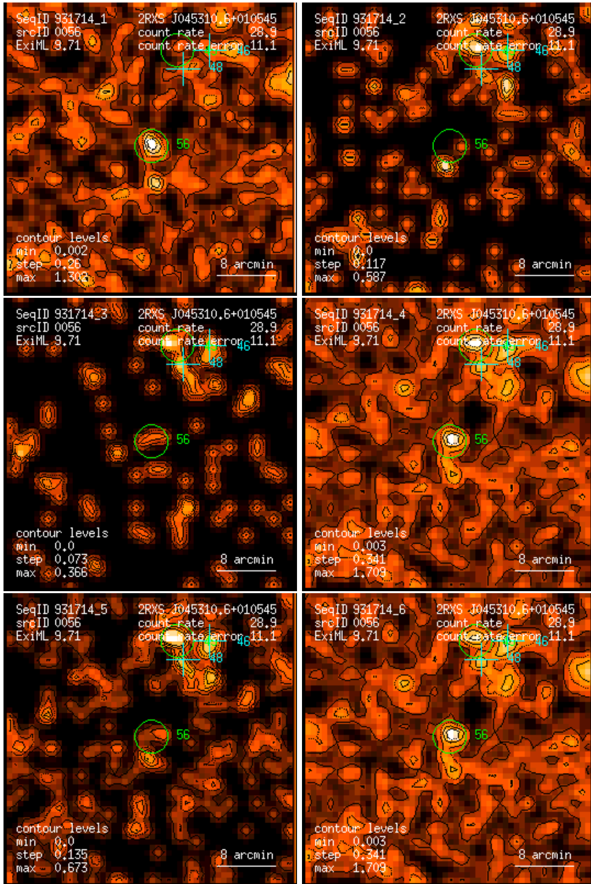
Figure 56: RASS 931714: detection 0056: band rate images, Gaussian filter: (1) PSPC channels 11 – 41, (2) 52 – 90, (3) 91 – 201, (4) 11 – 235, (5) 52 – 201, (6) 11 – 201. Broad band rates in counts/ks. Band rate contour levels in counts/ks/arcmin 2 .
