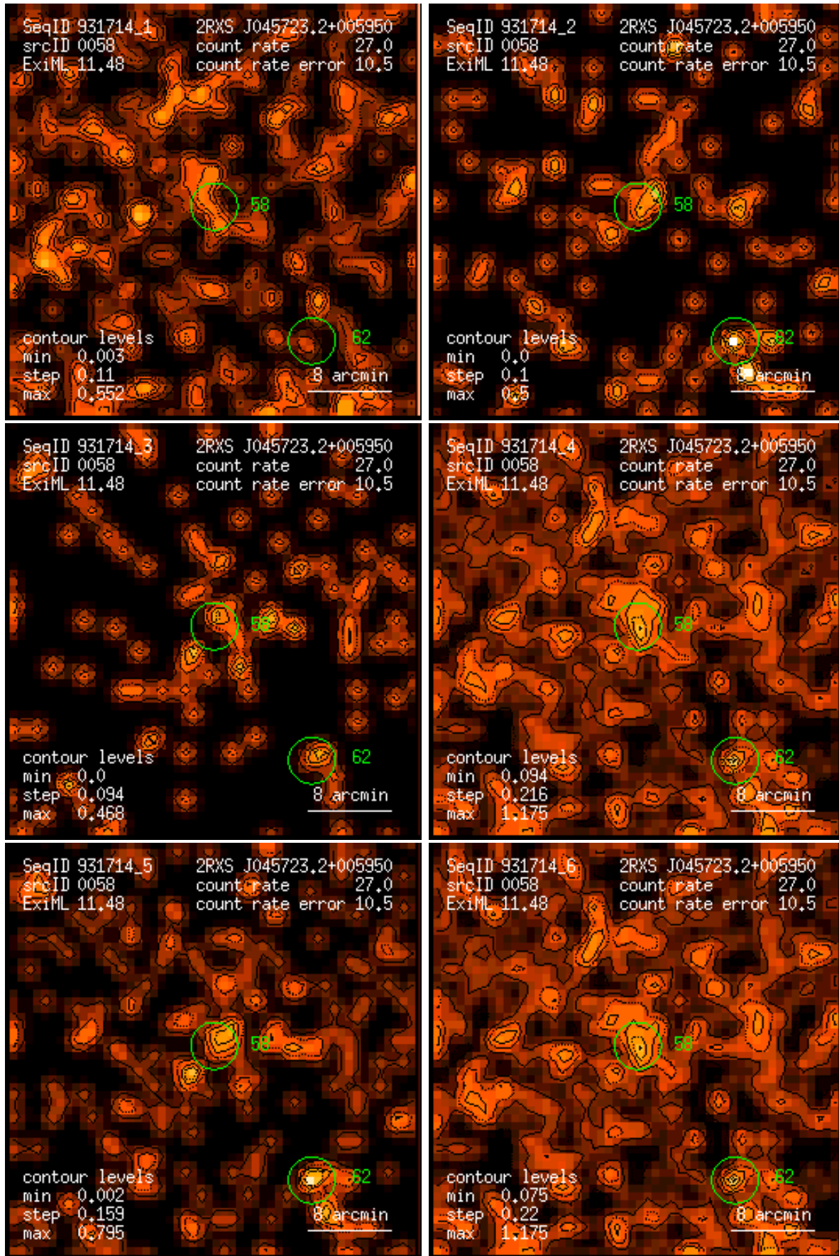
Figure 58: RASS 931714: detection 0058: band rate images, Gaussian filter: (1) PSPC channels 11 – 41, (2) 52 – 90, (3) 91 – 201, (4) 11 – 235, (5) 52 – 201, (6) 11 – 201. Broad band rates in counts/ks. Band rate contour levels in counts/ks/arcmin 2 .
