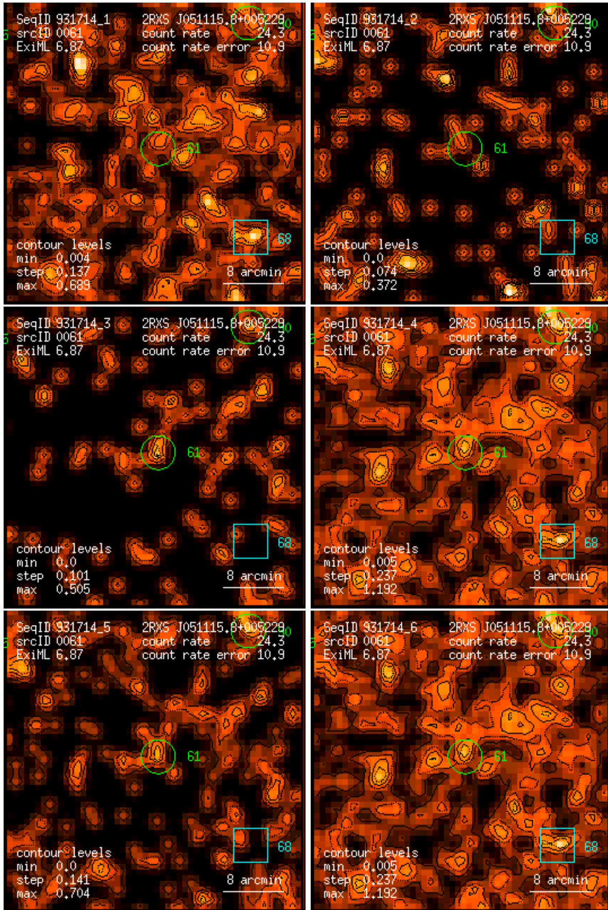
Figure 61: RASS 931714: detection 0061: band rate images, Gaussian filter: (1) PSPC channels 11 – 41, (2) 52 – 90, (3) 91 – 201, (4) 11 – 235, (5) 52 – 201, (6) 11 – 201. Broad band rates in counts/ks. Band rate contour levels in counts/ks/arcmin 2 .
