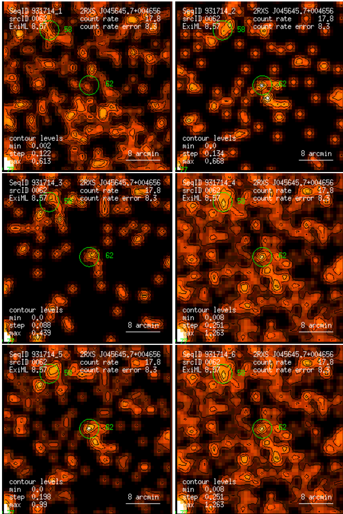
Figure 62: RASS 931714: detection 0062: band rate images, Gaussian filter: (1) PSPC channels 11 – 41, (2) 52 – 90, (3) 91 – 201, (4) 11 – 235, (5) 52 – 201, (6) 11 – 201. Broad band rates in counts/ks. Band rate contour levels in counts/ks/arcmin 2 .
