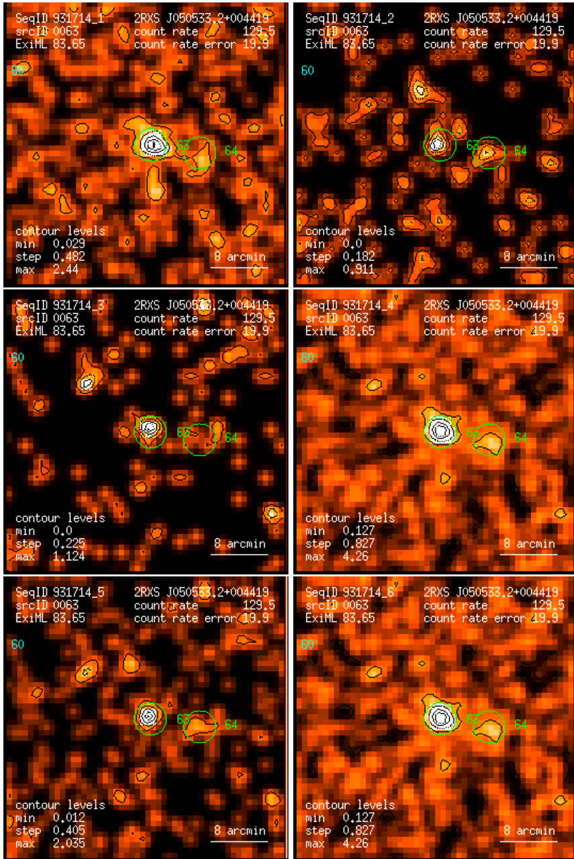
Figure 63: RASS 931714: detection 0063: band rate images, Gaussian filter: (1) PSPC channels 11 – 41, (2) 52 – 90, (3) 91 – 201, (4) 11 – 235, (5) 52 – 201, (6) 11 – 201. Broad band rates in counts/ks. Band rate contour levels in counts/ks/arcmin 2 .
