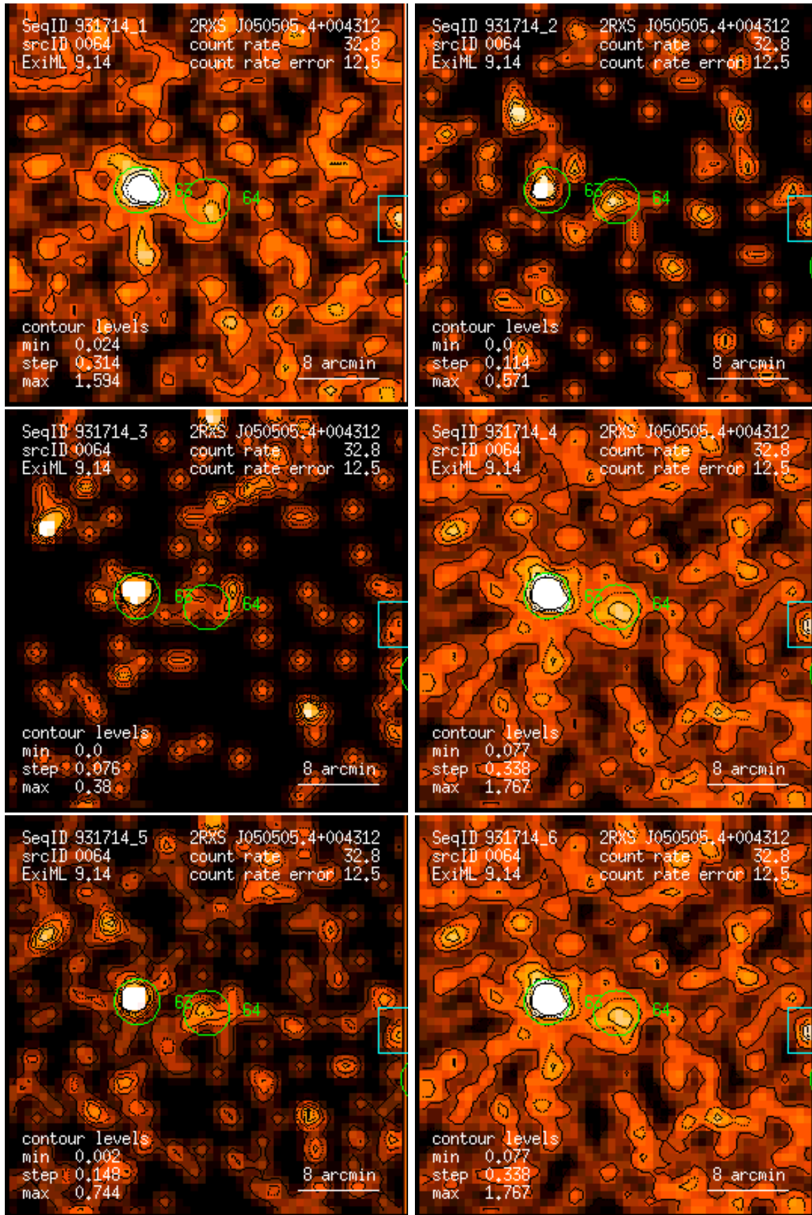
Figure 64: RASS 931714: detection 0064: band rate images, Gaussian filter: (1) PSPC channels 11 – 41, (2) 52 – 90, (3) 91 – 201, (4) 11 – 235, (5) 52 – 201, (6) 11 – 201. Broad band rates in counts/ks. Band rate contour levels in counts/ks/arcmin 2 .
