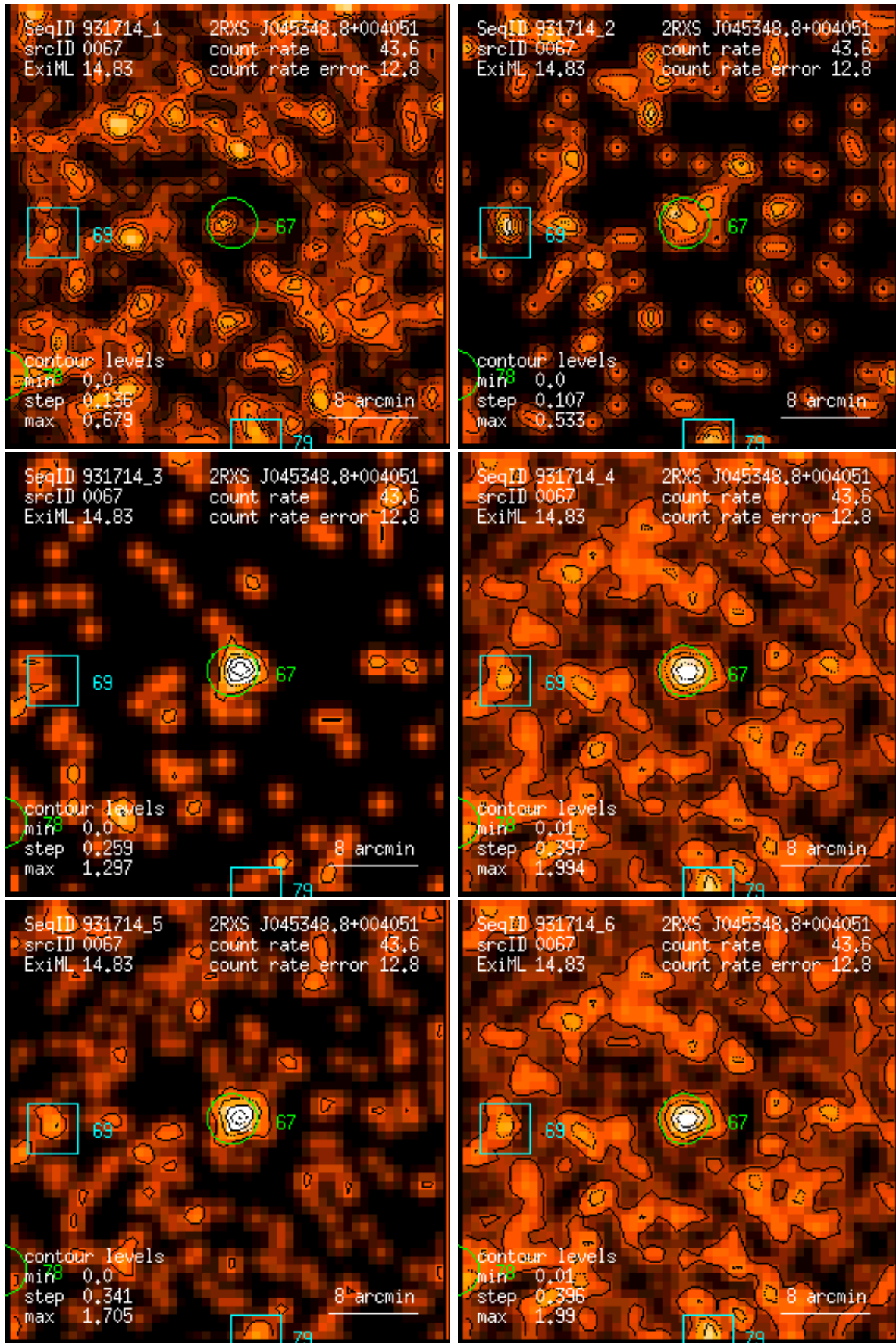
Figure 67: RASS 931714: detection 0067: band rate images, Gaussian filter: (1) PSPC channels 11 – 41, (2) 52 – 90, (3) 91 – 201, (4) 11 – 235, (5) 52 – 201, (6) 11 – 201. Broad band rates in counts/ks. Band rate contour levels in counts/ks/arcmin 2 .
