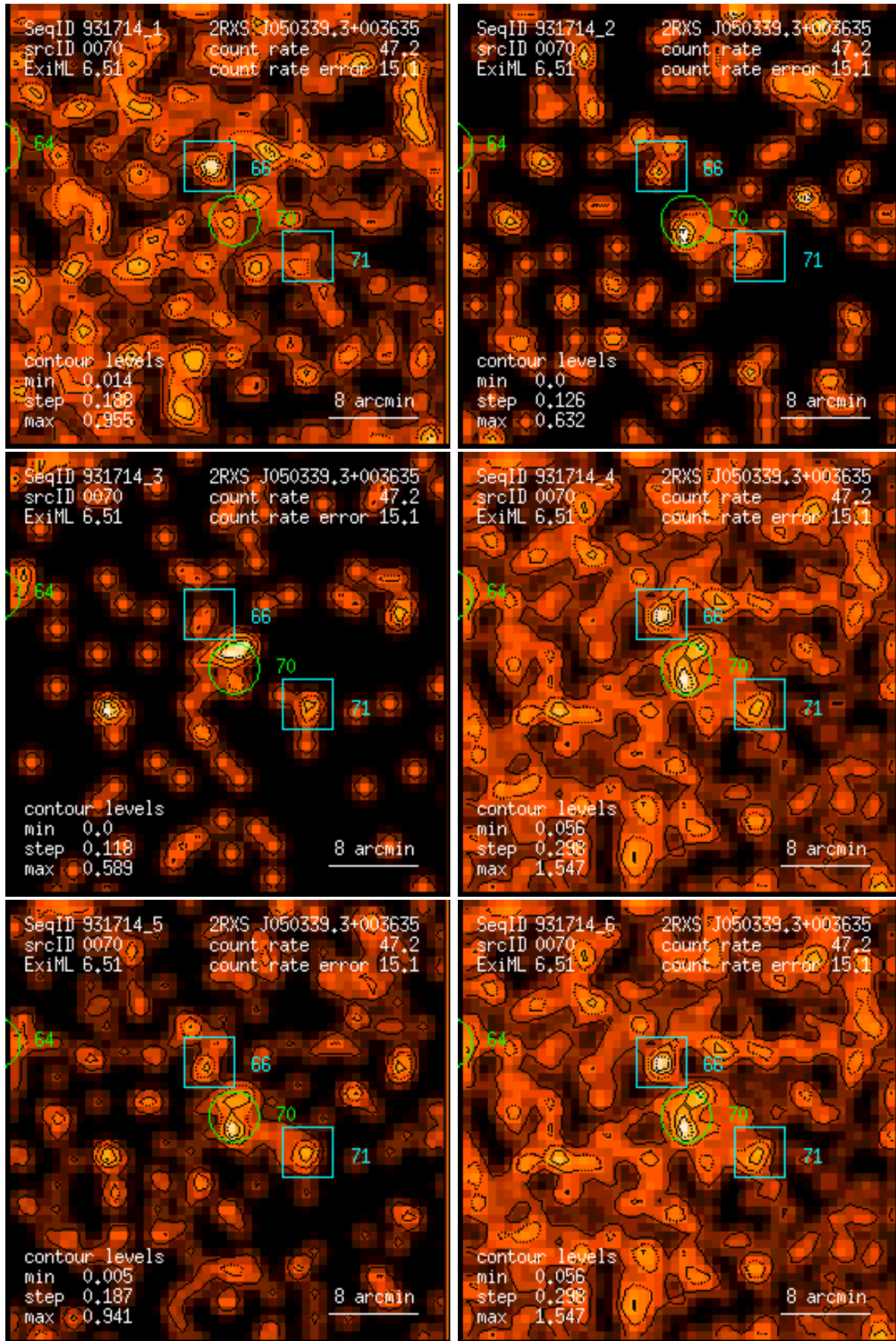
Figure 70: RASS 931714: detection 0070: band rate images, Gaussian filter: (1) PSPC channels 11 – 41, (2) 52 – 90, (3) 91 – 201, (4) 11 – 235, (5) 52 – 201, (6) 11 – 201. Broad band rates in counts/ks. Band rate contour levels in counts/ks/arcmin 2 .
