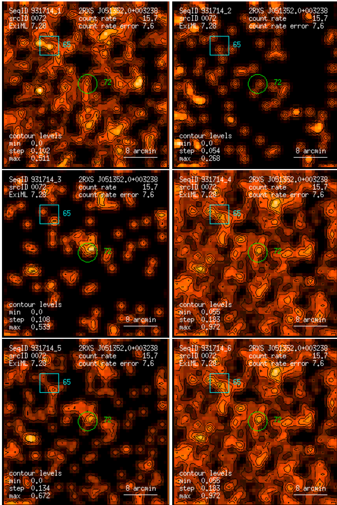
Figure 72: RASS 931714: detection 0072: band rate images, Gaussian filter: (1) PSPC channels 11 – 41, (2) 52 – 90, (3) 91 – 201, (4) 11 – 235, (5) 52 – 201, (6) 11 – 201. Broad band rates in counts/ks. Band rate contour levels in counts/ks/arcmin 2 .
