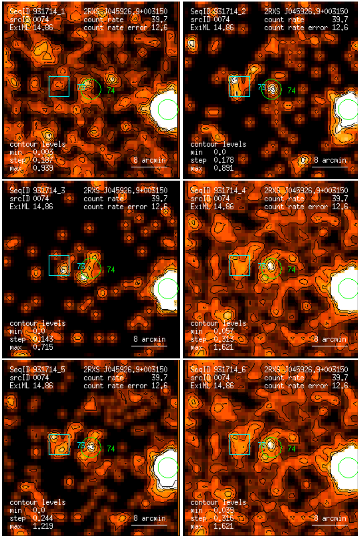
Figure 74: RASS 931714: detection 0074: band rate images, Gaussian filter: (1) PSPC channels 11 – 41, (2) 52 – 90, (3) 91 – 201, (4) 11 – 235, (5) 52 – 201, (6) 11 – 201. Broad band rates in counts/ks. Band rate contour levels in counts/ks/arcmin 2 .
