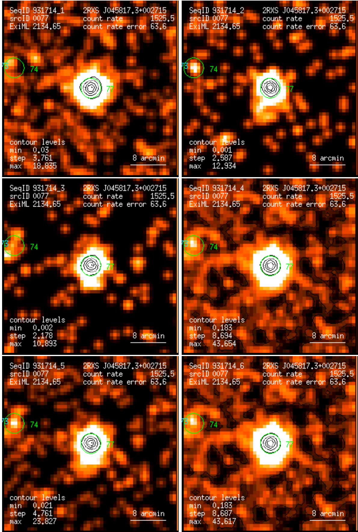
Figure 77: RASS 931714: detection 0077: band rate images, Gaussian filter: (1) PSPC channels 11 – 41, (2) 52 – 90, (3) 91 – 201, (4) 11 – 235, (5) 52 – 201, (6) 11 – 201. Broad band rates in counts/ks. Band rate contour levels in counts/ks/arcmin 2 .
