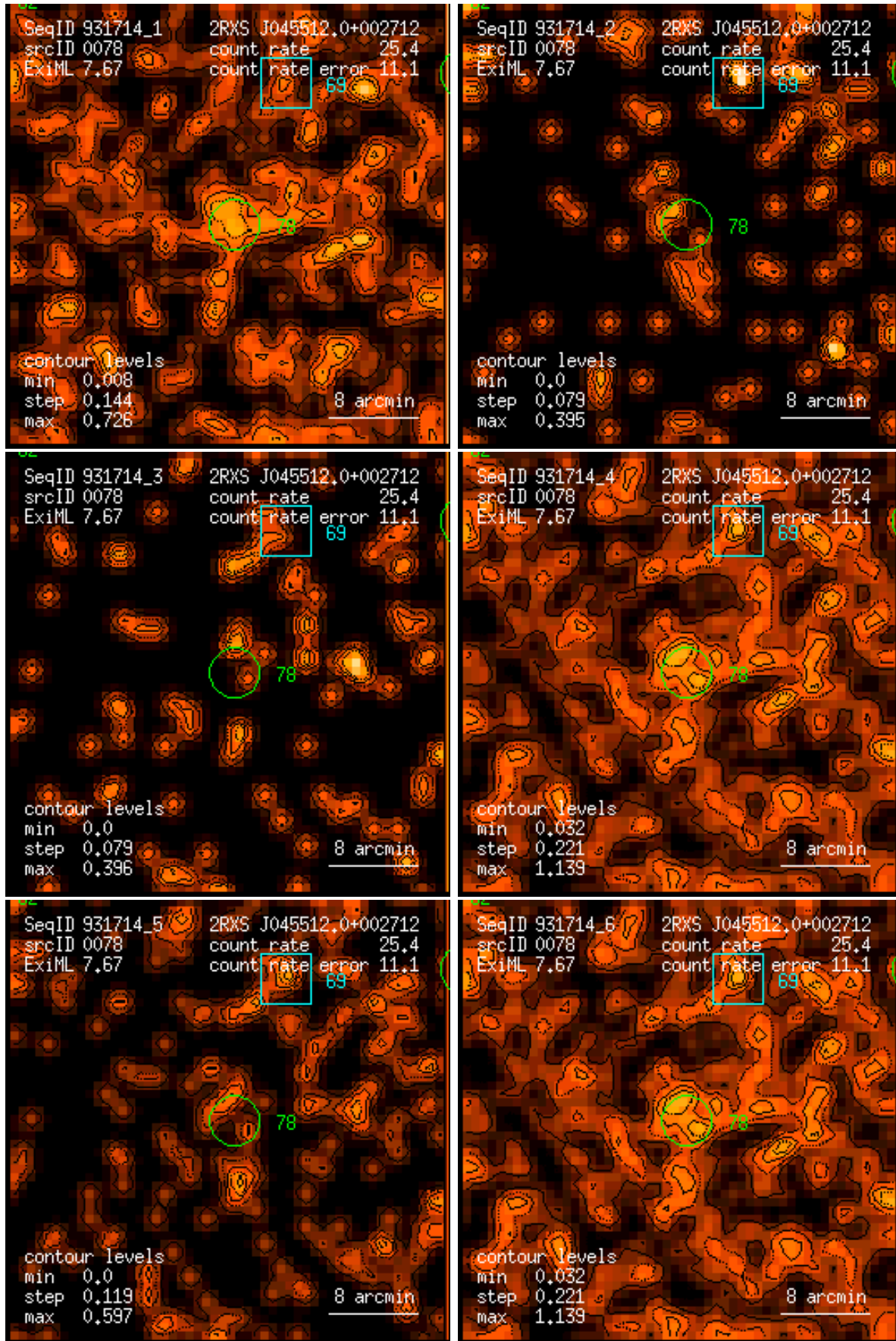
Figure 78: RASS 931714: detection 0078: band rate images, Gaussian filter: (1) PSPC channels 11 – 41, (2) 52 – 90, (3) 91 – 201, (4) 11 – 235, (5) 52 – 201, (6) 11 – 201. Broad band rates in counts/ks. Band rate contour levels in counts/ks/arcmin 2 .
