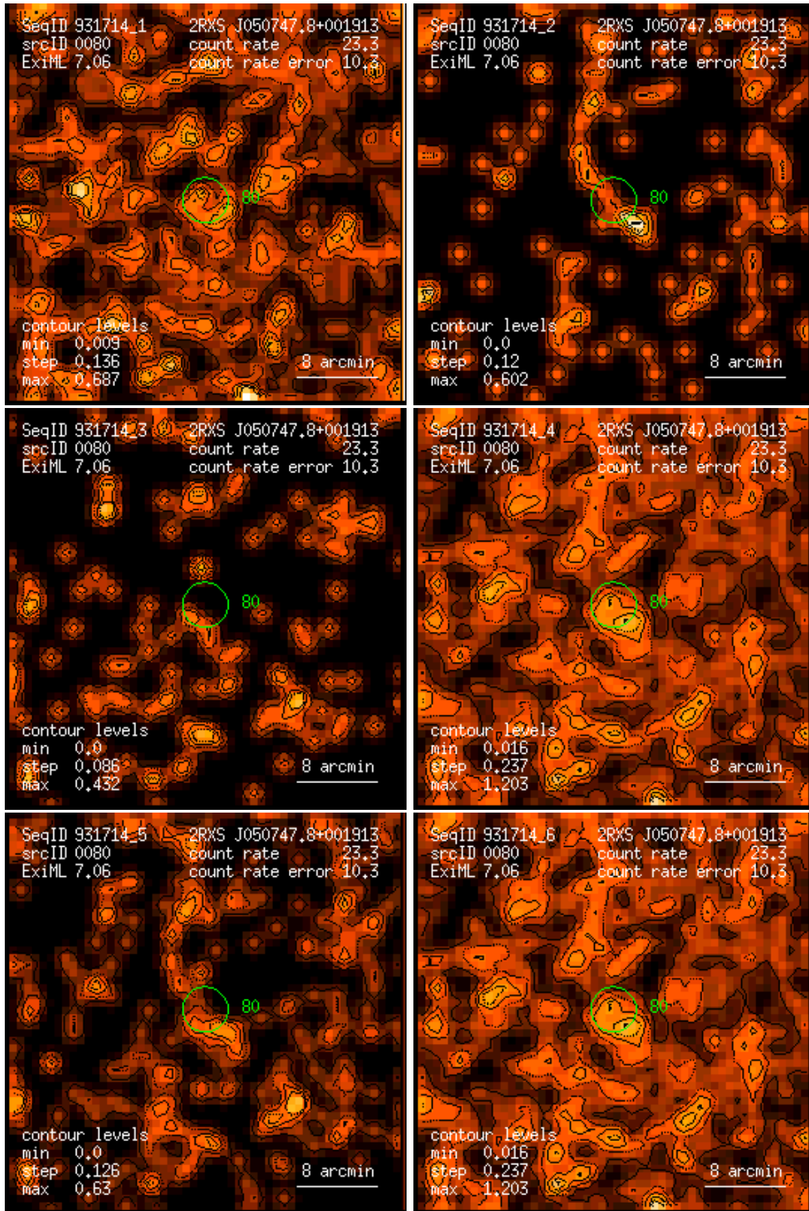
Figure 80: RASS 931714: detection 0080: band rate images, Gaussian filter: (1) PSPC channels 11 – 41, (2) 52 – 90, (3) 91 – 201, (4) 11 – 235, (5) 52 – 201, (6) 11 – 201. Broad band rates in counts/ks. Band rate contour levels in counts/ks/arcmin 2 .
