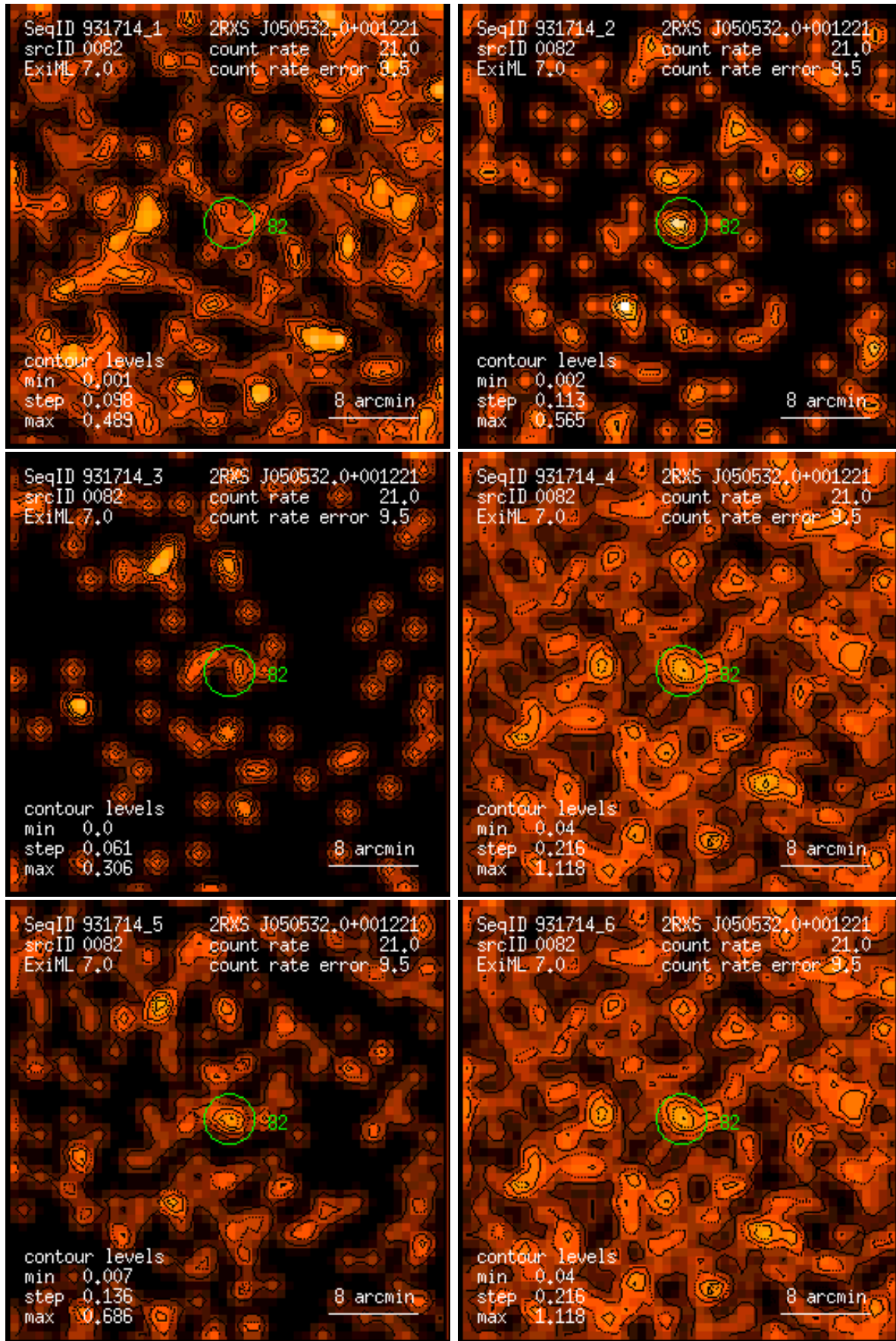
Figure 82: RASS 931714: detection 0082: band rate images, Gaussian filter: (1) PSPC channels 11 – 41, (2) 52 – 90, (3) 91 – 201, (4) 11 – 235, (5) 52 – 201, (6) 11 – 201. Broad band rates in counts/ks. Band rate contour levels in counts/ks/arcmin 2 .
