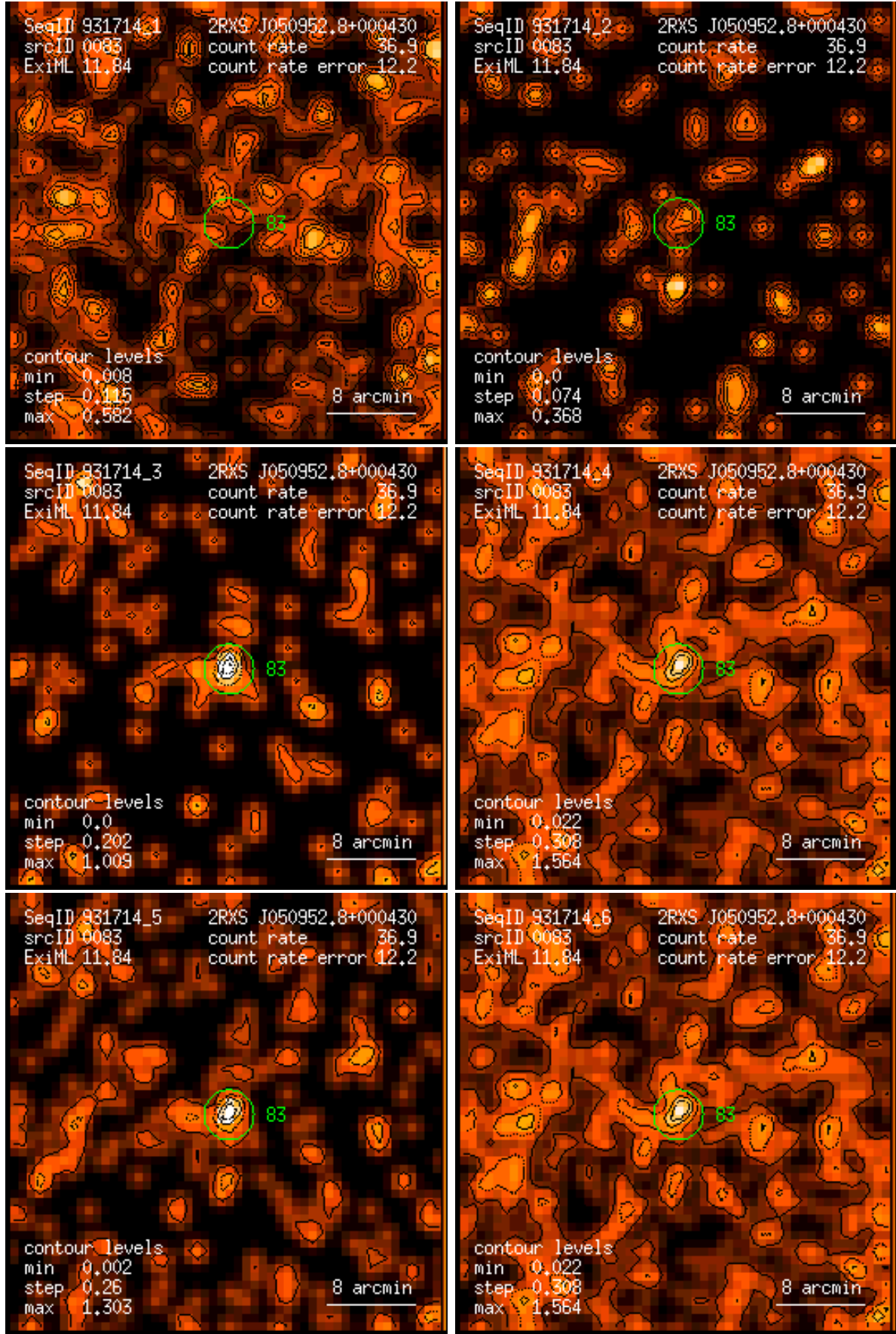
Figure 83: RASS 931714: detection 0083: band rate images, Gaussian filter: (1) PSPC channels 11 – 41, (2) 52 – 90, (3) 91 – 201, (4) 11 – 235, (5) 52 – 201, (6) 11 – 201. Broad band rates in counts/ks. Band rate contour levels in counts/ks/arcmin 2 .
