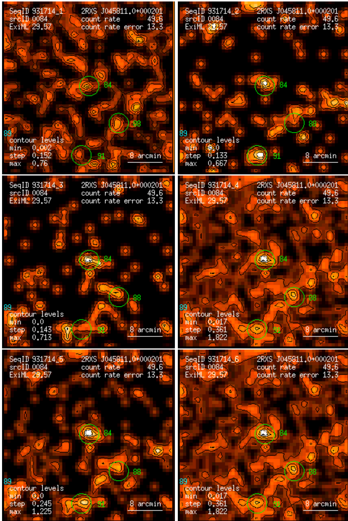
Figure 84: RASS 931714: detection 0084: band rate images, Gaussian filter: (1) PSPC channels 11 – 41, (2) 52 – 90, (3) 91 – 201, (4) 11 – 235, (5) 52 – 201, (6) 11 – 201. Broad band rates in counts/ks. Band rate contour levels in counts/ks/arcmin 2 .
