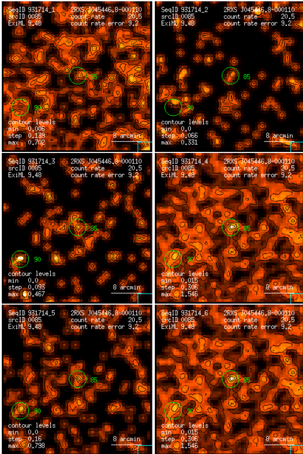
Figure 85: RASS 931714: detection 0085: band rate images, Gaussian filter: (1) PSPC channels 11 – 41, (2) 52 – 90, (3) 91 – 201, (4) 11 – 235, (5) 52 – 201, (6) 11 – 201. Broad band rates in counts/ks. Band rate contour levels in counts/ks/arcmin 2 .
