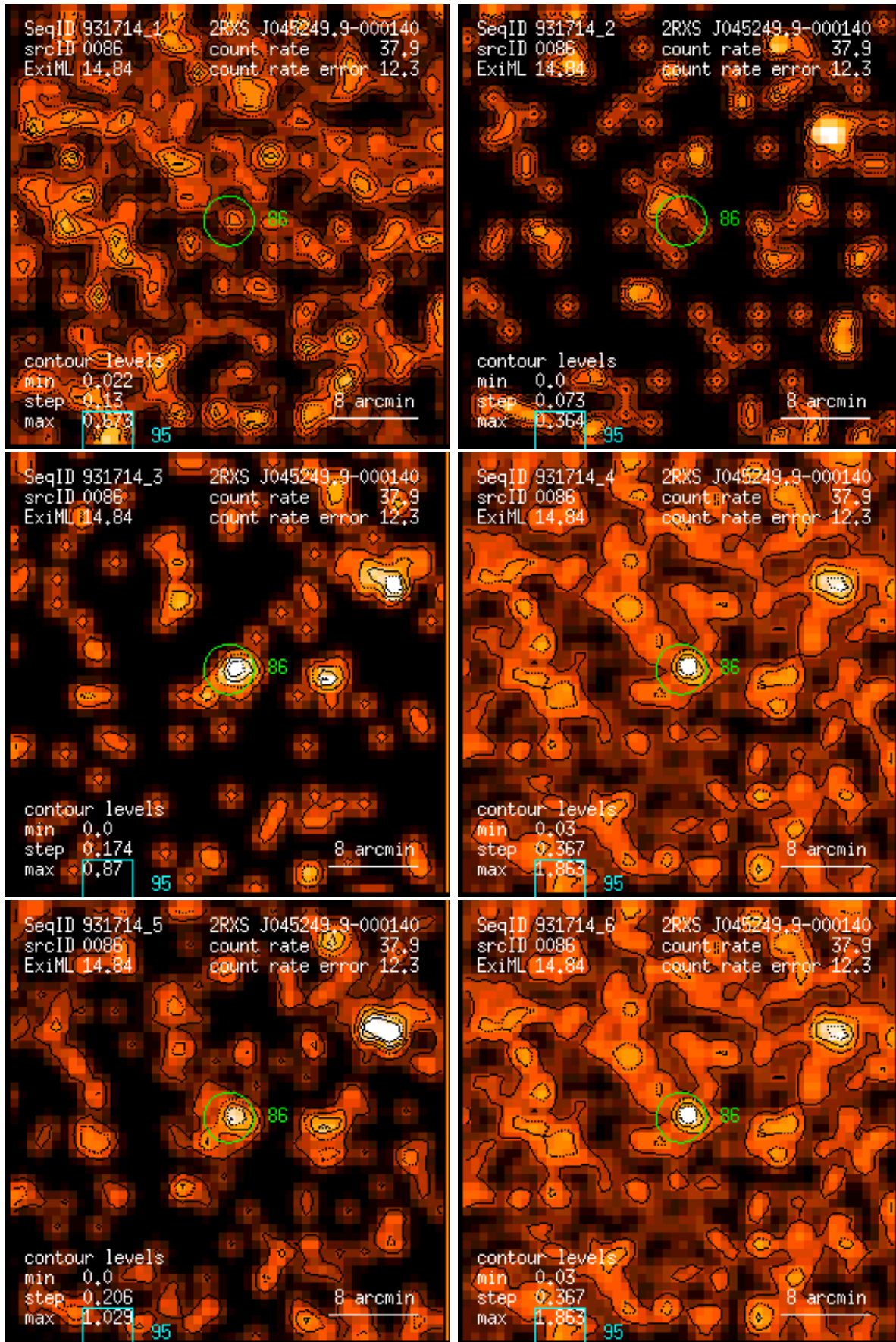
Figure 86: RASS 931714: detection 0086: band rate images, Gaussian filter: (1) PSPC channels 11 – 41, (2) 52 – 90, (3) 91 – 201, (4) 11 – 235, (5) 52 – 201, (6) 11 – 201. Broad band rates in counts/ks. Band rate contour levels in counts/ks/arcmin 2 .
