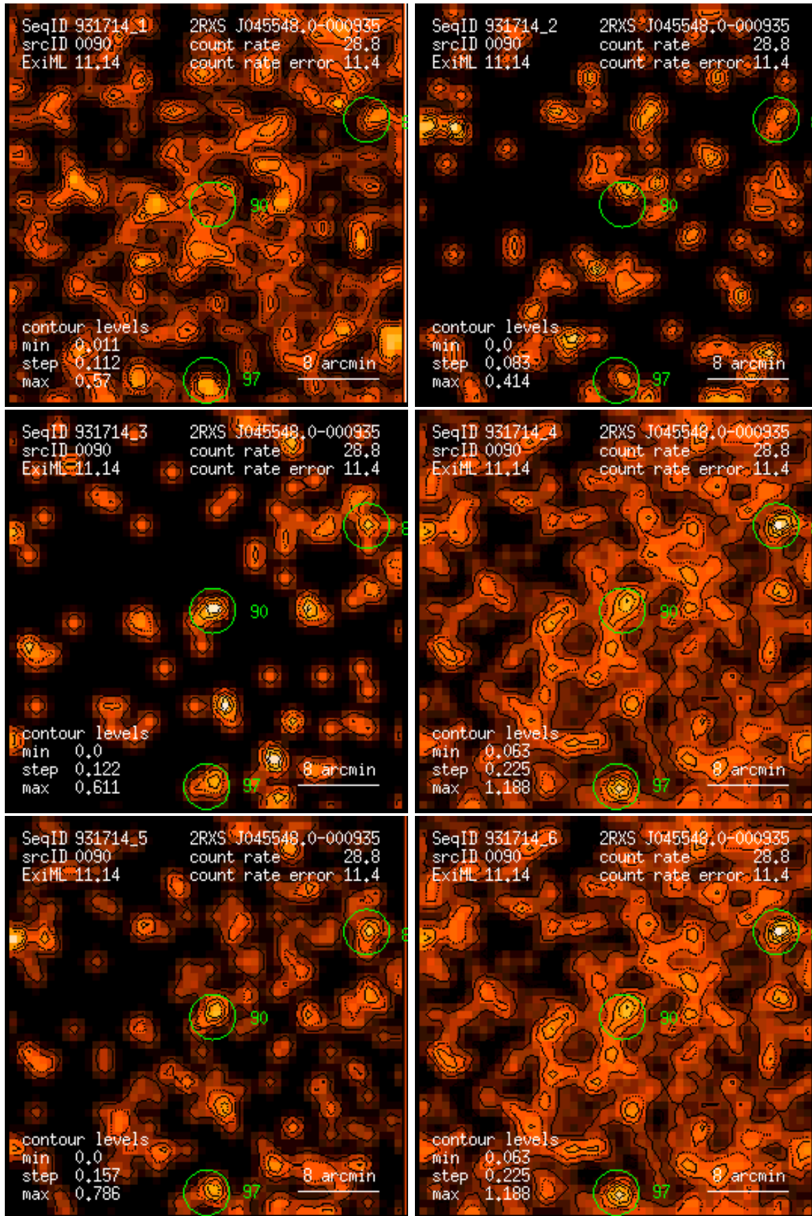
Figure 90: RASS 931714: detection 0090: band rate images, Gaussian filter: (1) PSPC channels 11 – 41, (2) 52 – 90, (3) 91 – 201, (4) 11 – 235, (5) 52 – 201, (6) 11 – 201. Broad band rates in counts/ks. Band rate contour levels in counts/ks/arcmin 2 .
