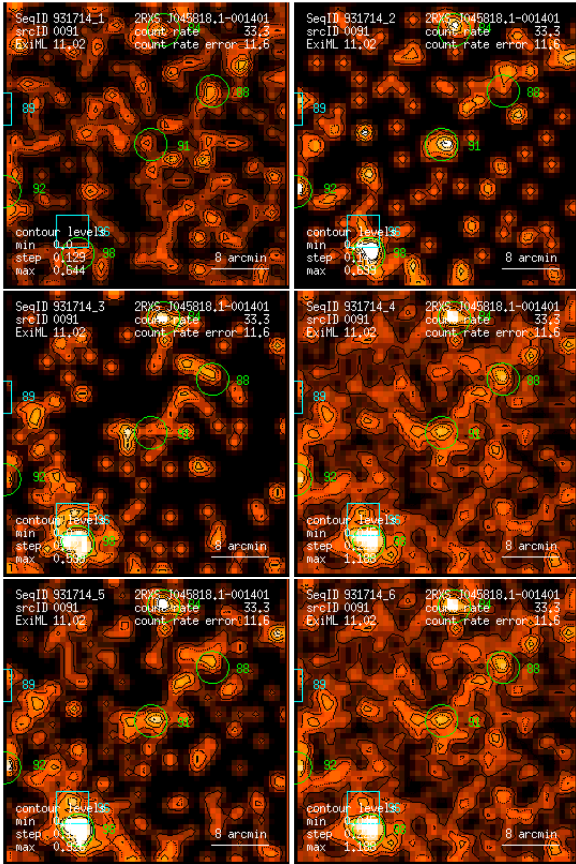
Figure 91: RASS 931714: detection 0091: band rate images, Gaussian filter: (1) PSPC channels 11 – 41, (2) 52 – 90, (3) 91 – 201, (4) 11 – 235, (5) 52 – 201, (6) 11 – 201. Broad band rates in counts/ks. Band rate contour levels in counts/ks/arcmin 2 .
