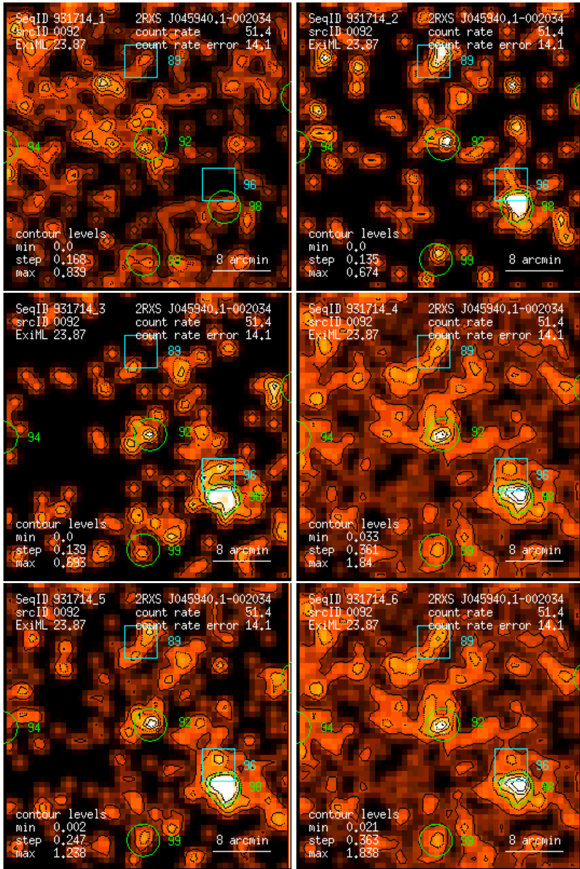
Figure 92: RASS 931714: detection 0092: band rate images, Gaussian filter: (1) PSPC channels 11 – 41, (2) 52 – 90, (3) 91 – 201, (4) 11 – 235, (5) 52 – 201, (6) 11 – 201. Broad band rates in counts/ks. Band rate contour levels in counts/ks/arcmin 2 .
