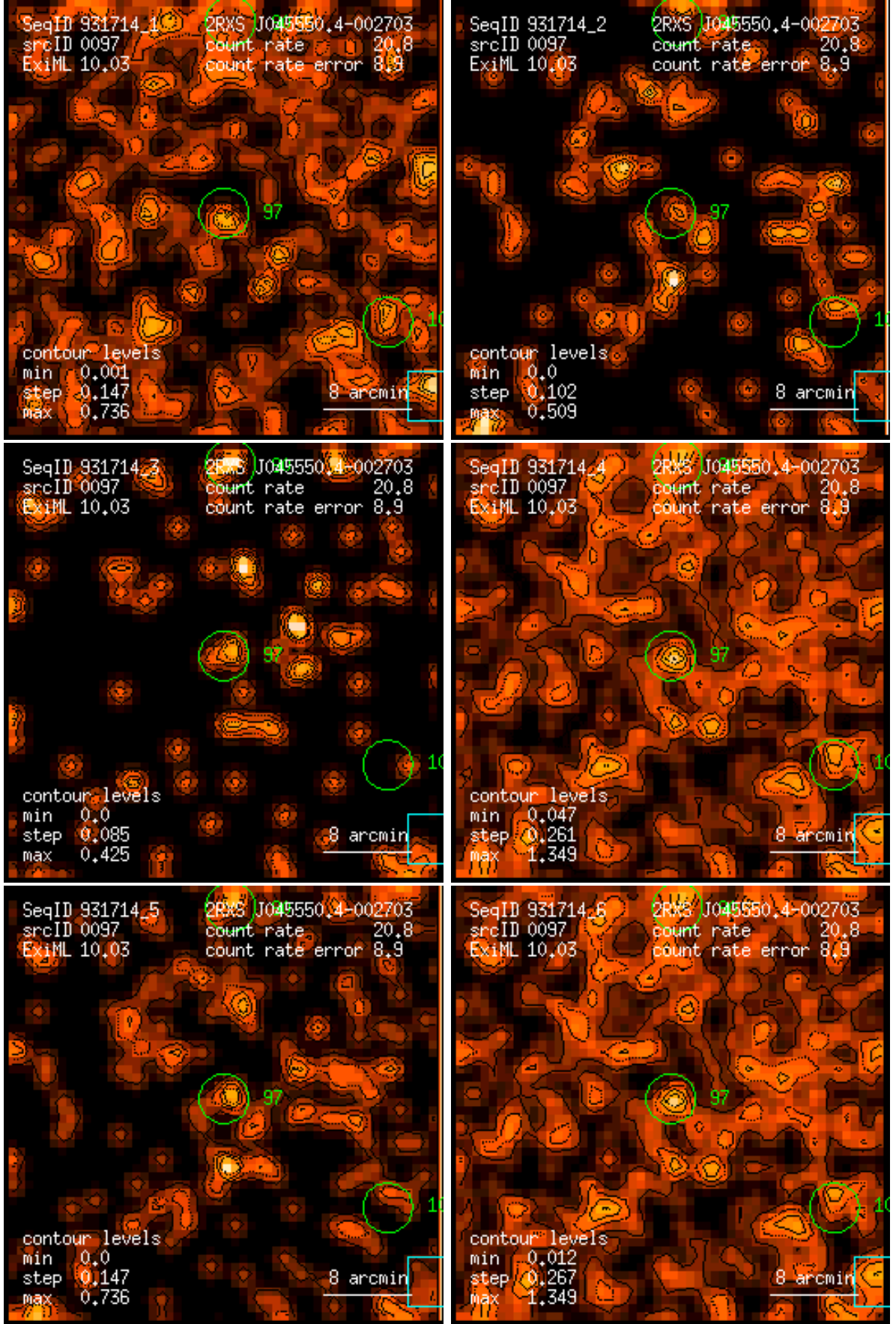
Figure 97: RASS 931714: detection 0097: band rate images, Gaussian filter: (1) PSPC channels 11 – 41, (2) 52 – 90, (3) 91 – 201, (4) 11 – 235, (5) 52 – 201, (6) 11 – 201. Broad band rates in counts/ks. Band rate contour levels in counts/ks/arcmin 2 .
