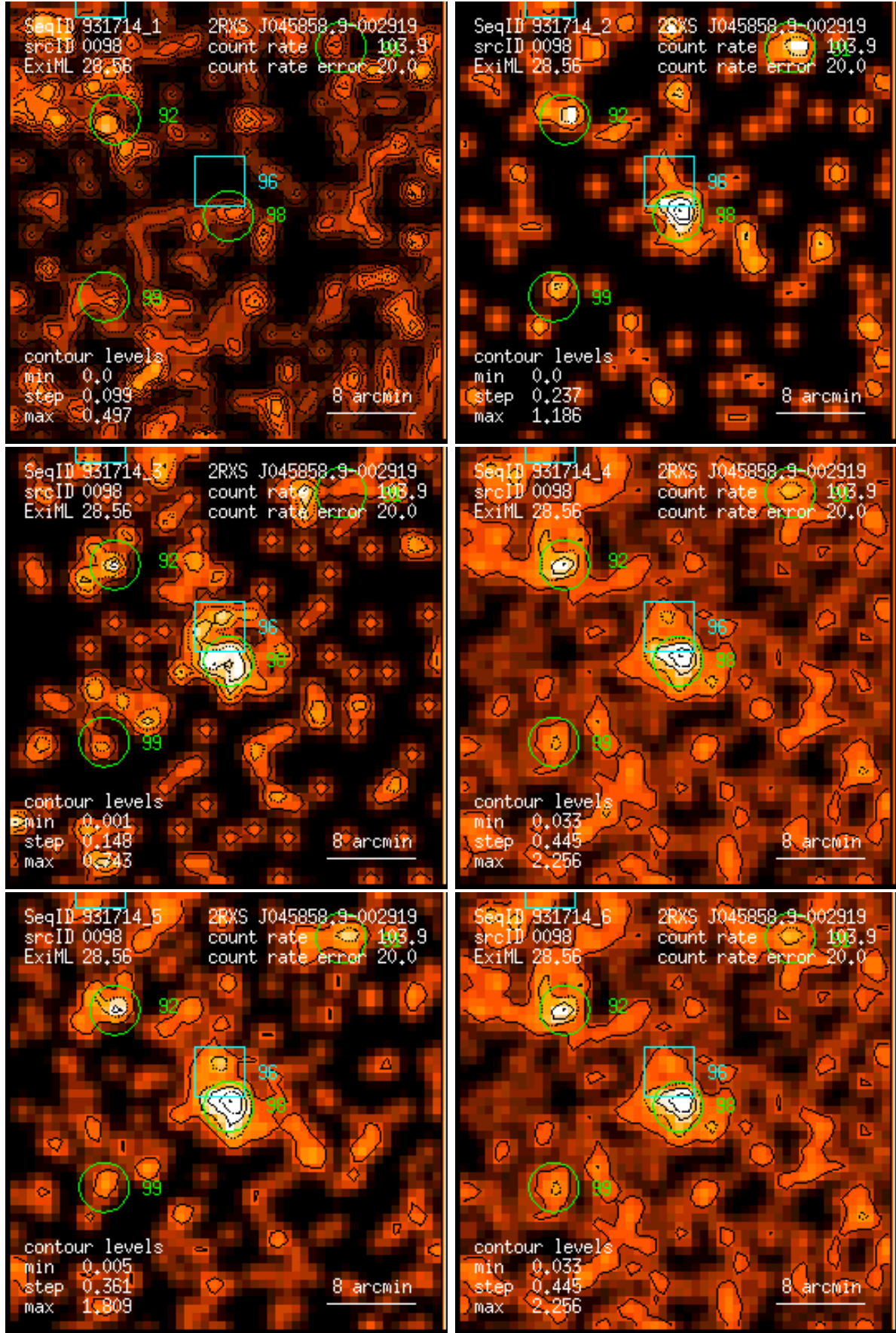
Figure 98: RASS 931714: detection 0098: band rate images, Gaussian filter: (1) PSPC channels 11 – 41, (2) 52 – 90, (3) 91 – 201, (4) 11 – 235, (5) 52 – 201, (6) 11 – 201. Broad band rates in counts/ks. Band rate contour levels in counts/ks/arcmin 2 .
