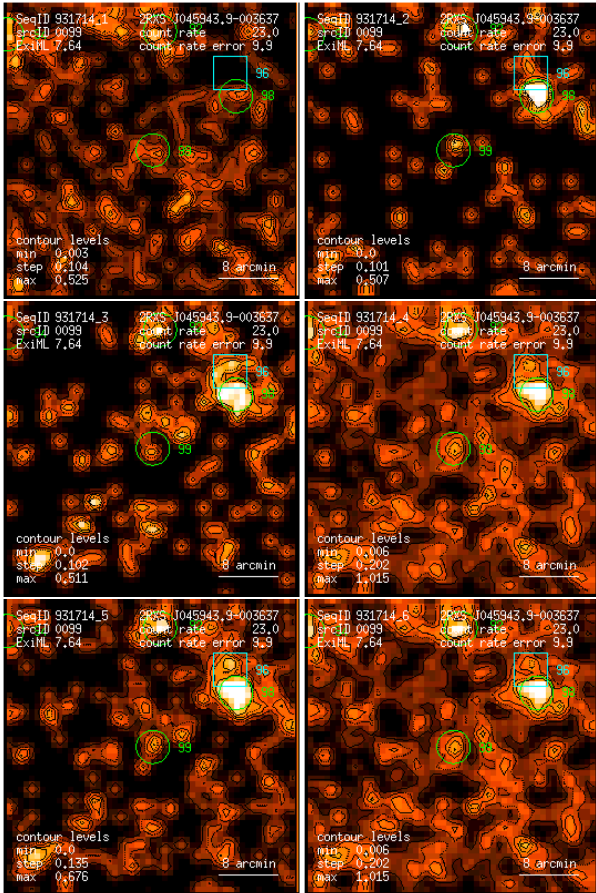
Figure 99: RASS 931714: detection 0099: band rate images, Gaussian filter: (1) PSPC channels 11 – 41, (2) 52 – 90, (3) 91 – 201, (4) 11 – 235, (5) 52 – 201, (6) 11 – 201. Broad band rates in counts/ks. Band rate contour levels in counts/ks/arcmin 2 .
