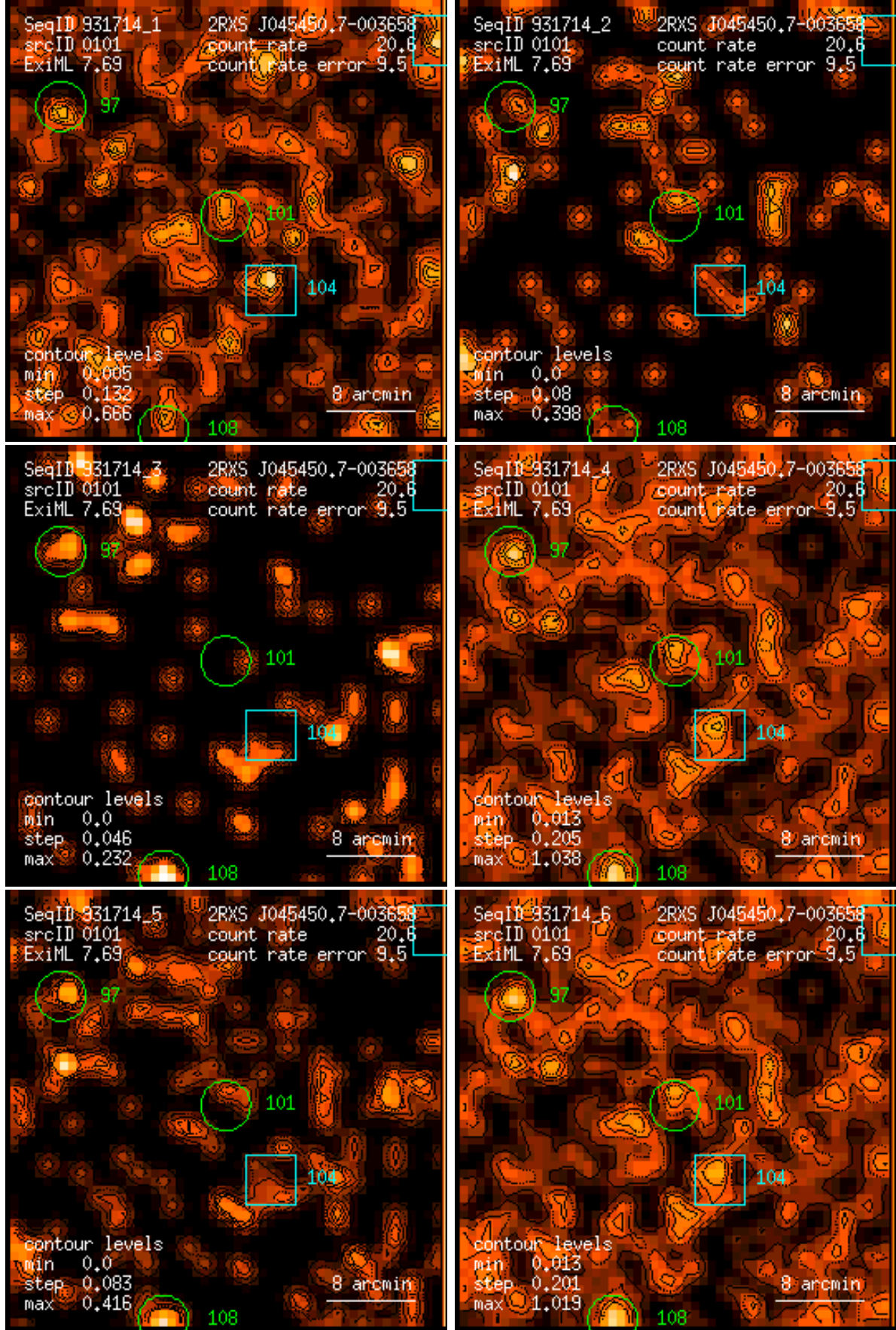
Figure 101: RASS 931714: detection 0101: band rate images, Gaussian filter: (1) PSPC channels 11 – 41, (2) 52 – 90, (3) 91 – 201, (4) 11 – 235, (5) 52 – 201, (6) 11 – 201. Broad band rates in counts/ks. Band rate contour levels in counts/ks/arcmin 2 .
